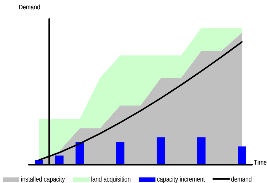
Figure 8.5: Demand/Capacity Model of Water Supply Delivery Infrastructure
