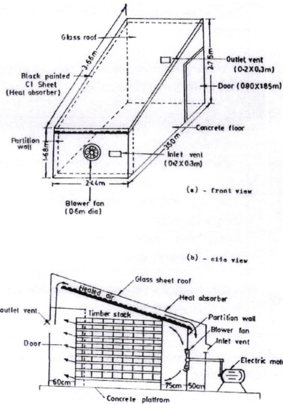
Figure 2. A schematic diagram of a 3.5 m 3 capacity solar kiln
