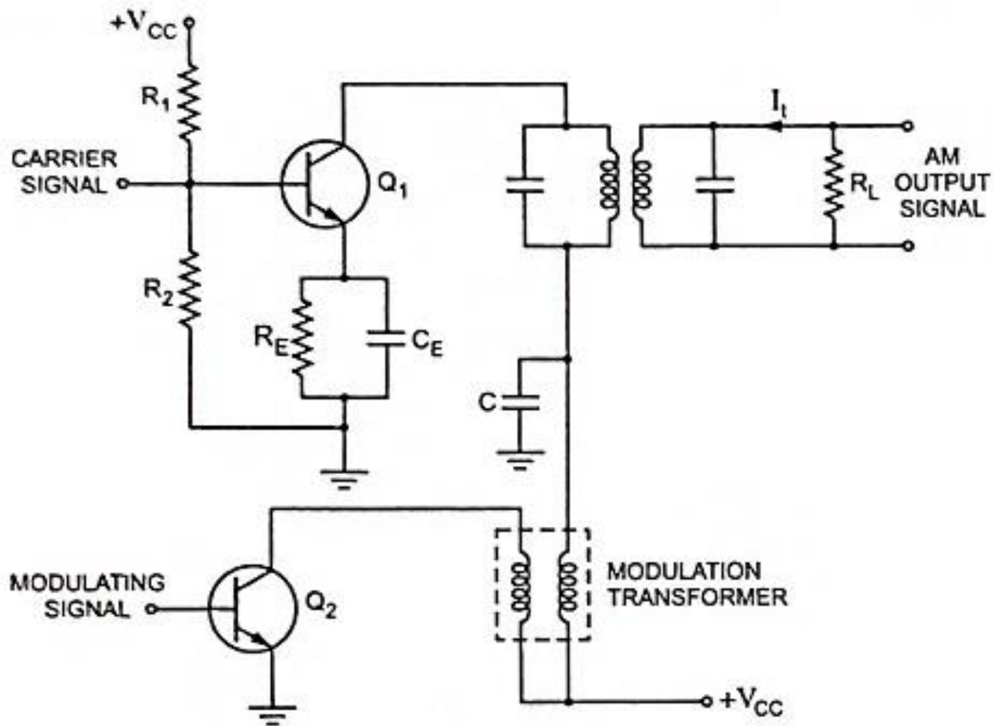
Fig. 22.26 Collector Modulation Circuit
