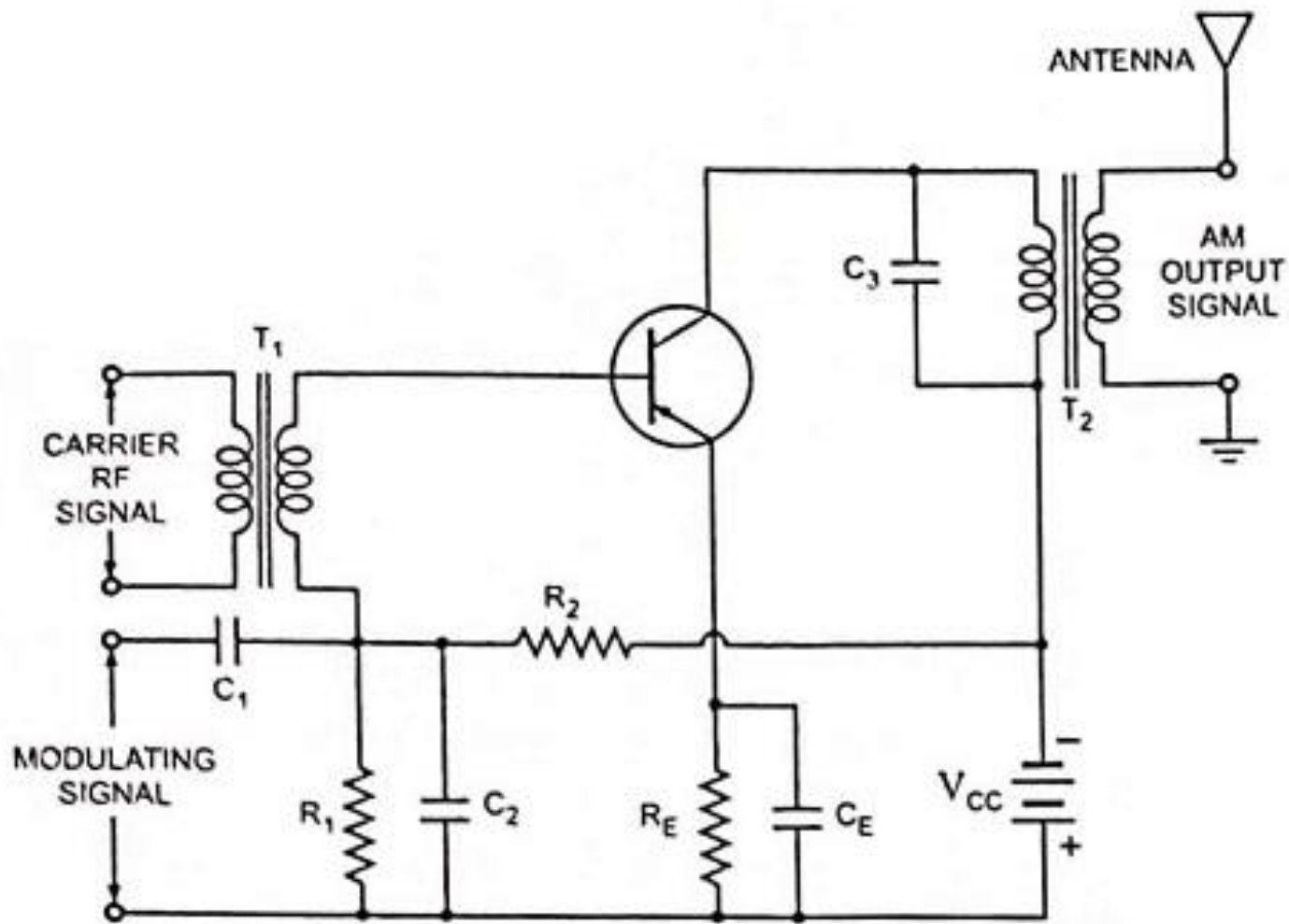
Fig. 22.28 Base Modulation Circuit
