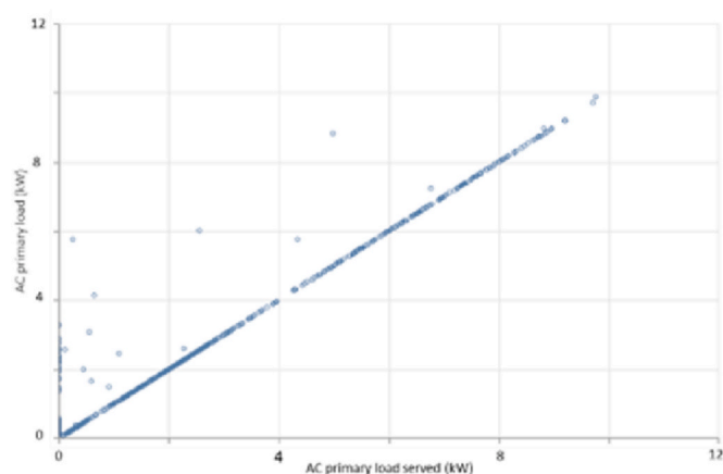
Fig. A2. Load serving capability of the proposed 28 kWp PV-battery AC plant in Imvepi trading centre, Uganda.
