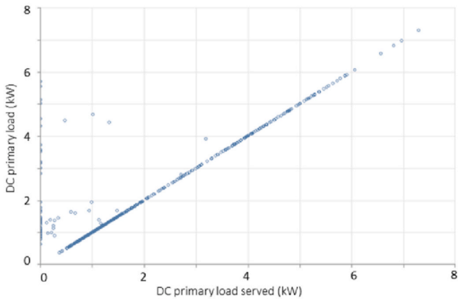
Fig. A5. Load serving capability of the proposed 16 kWp PV-battery DC power plant for refugee households in Bangladesh.
