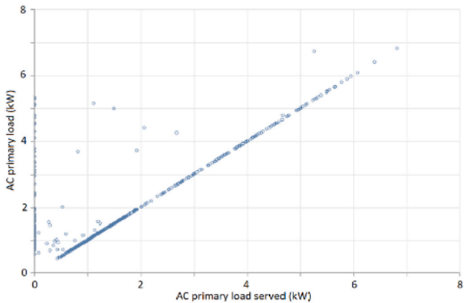
Fig. A4. Load serving capability of the proposed 20 kWp PV-battery AC power plant for refugee households in Bangladesh.
