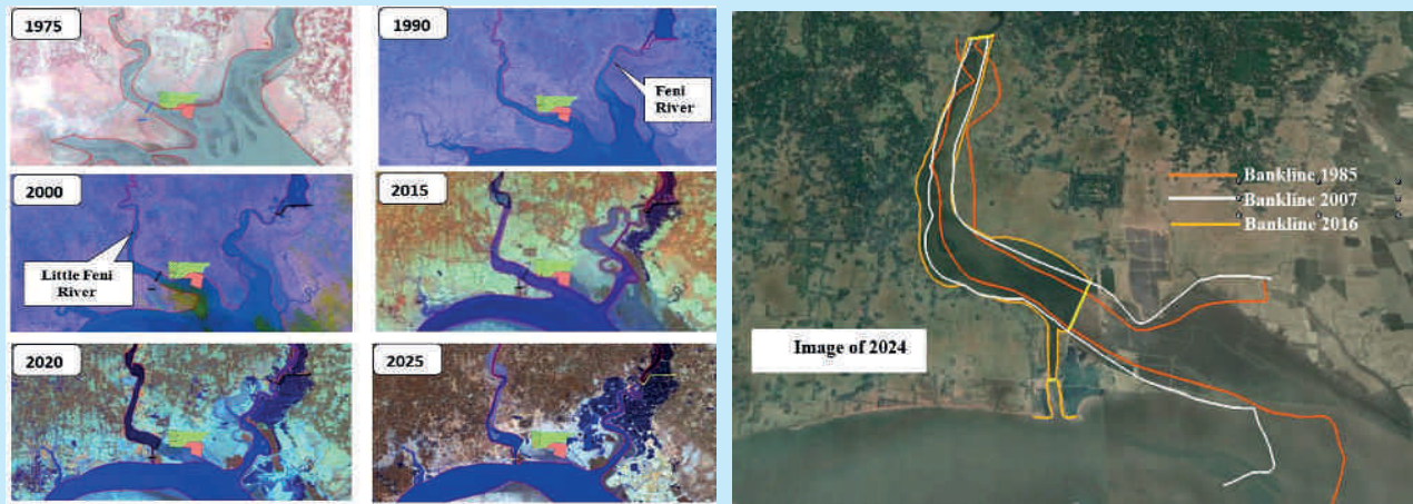
Figure 1: Historical river channel positions at and around the project area
