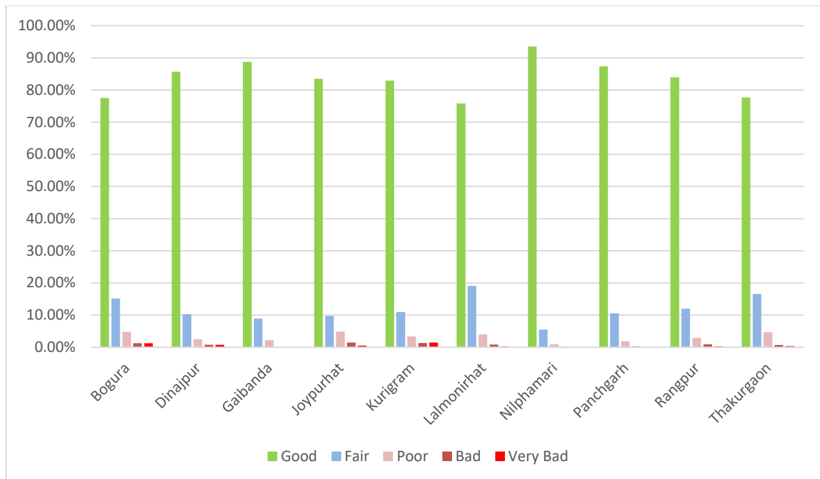
Figure 3.14: Road Condition (%) of Rangpur Zone based on IRI Data
