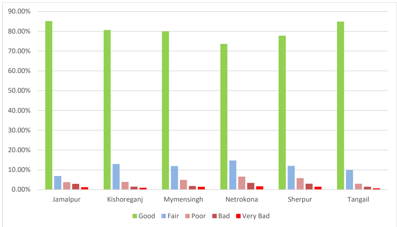
Figure 3.12: Road Condition (%) of Mymensingh Zone based on IRI Data
