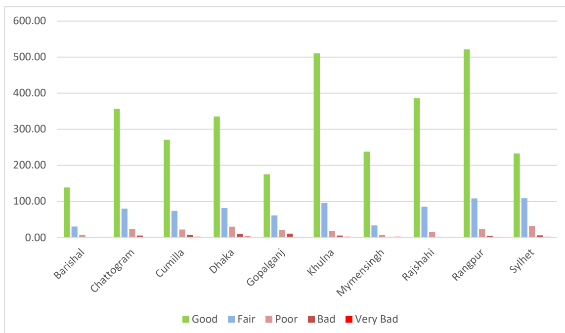
Figure 3.3: Road Condition (in km) of National Highways based on IRI Data
