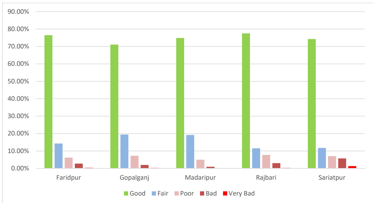
Figure 3.10: Road Condition (%) of Gopalganj Zone based on IRI Data
