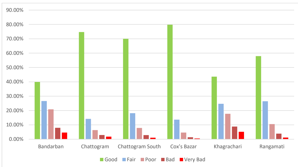
Figure: 3.7: Road Condition (%) of Chattogram Zone based on IRI
