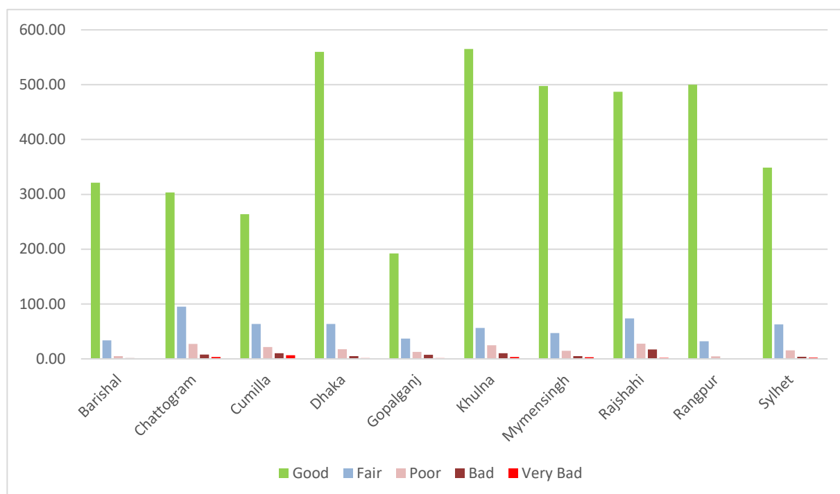
Figure 3.4: Road Condition (in km) of Regional Highways based on IRI Data
