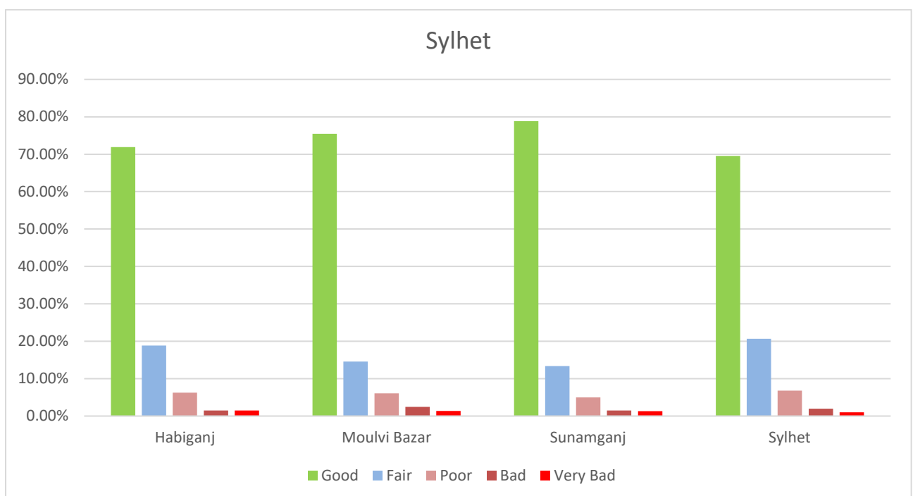
Figure 3.15: Road Condition (%) of Sylhet Zone based on IRI Data
