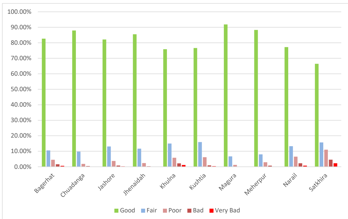
Figure 3.11: Road Condition (%) of Khulna Zone based on IRI Data
