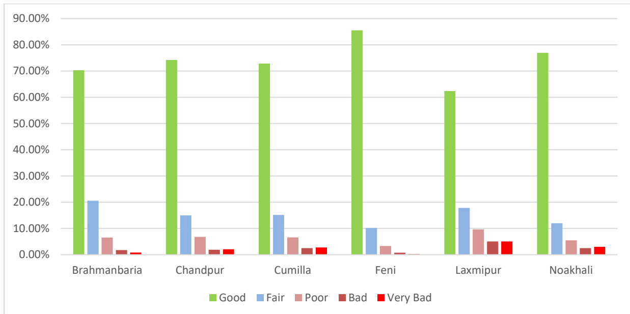
Figure 3.8: Road Condition (%) of Cumilla Zone based on IRI Data
