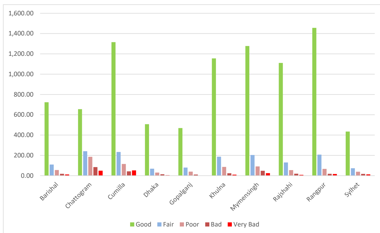
Figure 3.5: Road Condition (in km) of Zilla Highways based on IRI Data
