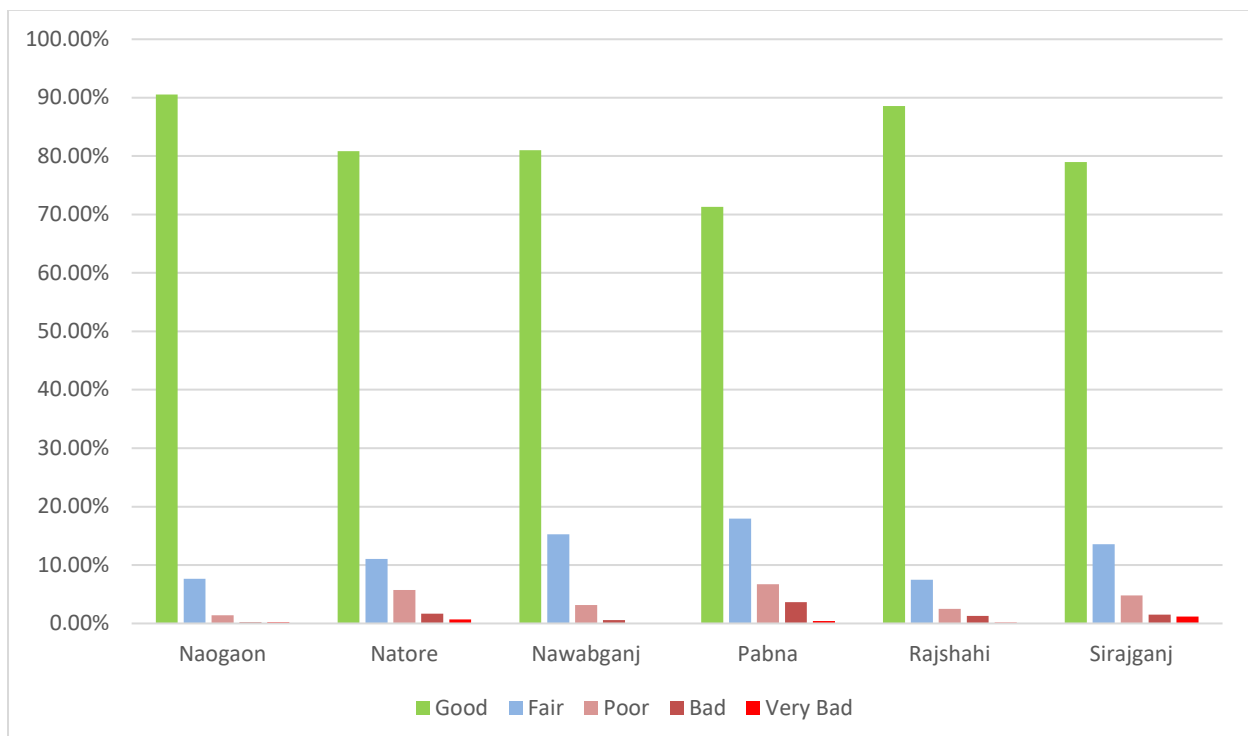
Figure 3.13: Road Condition (%) of Rajshahi Zone based on IRI Data
