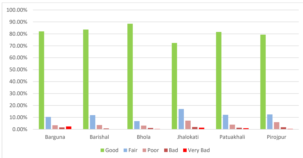
Figure: 3.6: Road Condition (%) of Barishal Zone based on IRI Data
