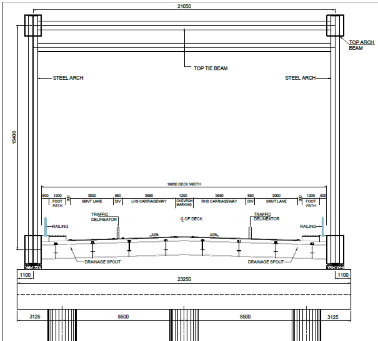
Figure 4-2: Cross Section of Steel Arch bridge
