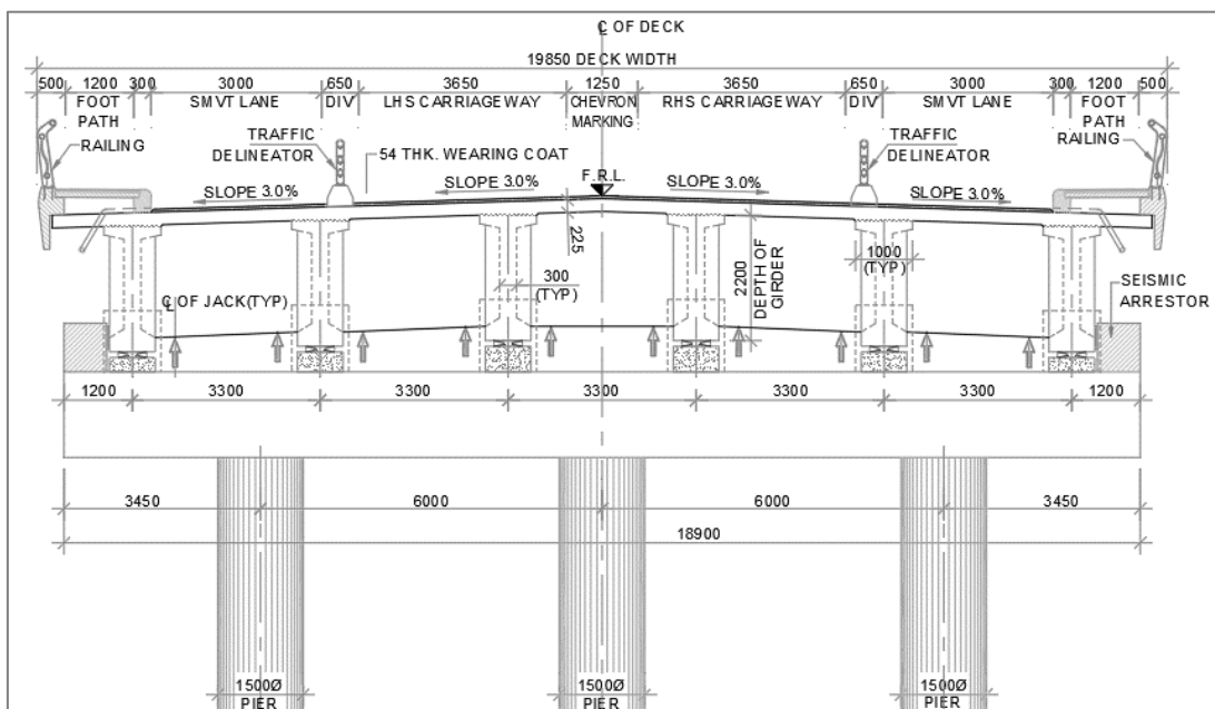
Figure 4-3: Cross Section of PSC I-Girder Type Viaduct
