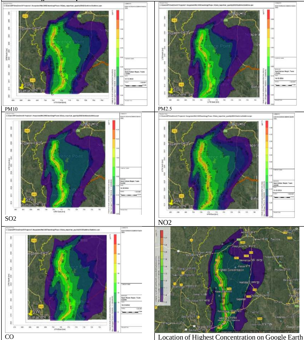
Figure 7-2: Isoleths of Predicted Concentration of Criteria Pollutants in Ambient Air
