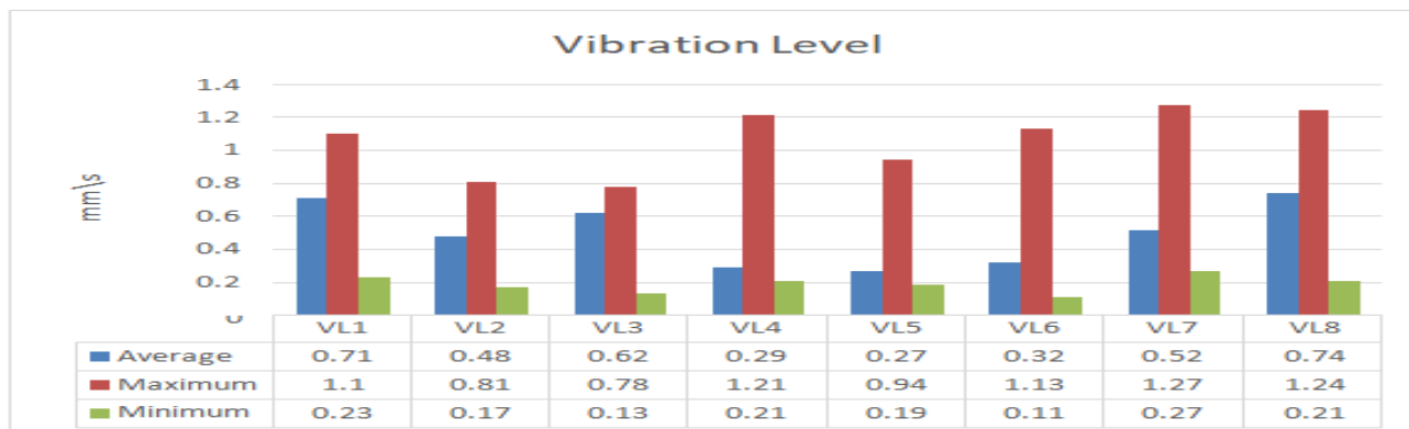
Figure 4-18: Vibration Monitoring Results
