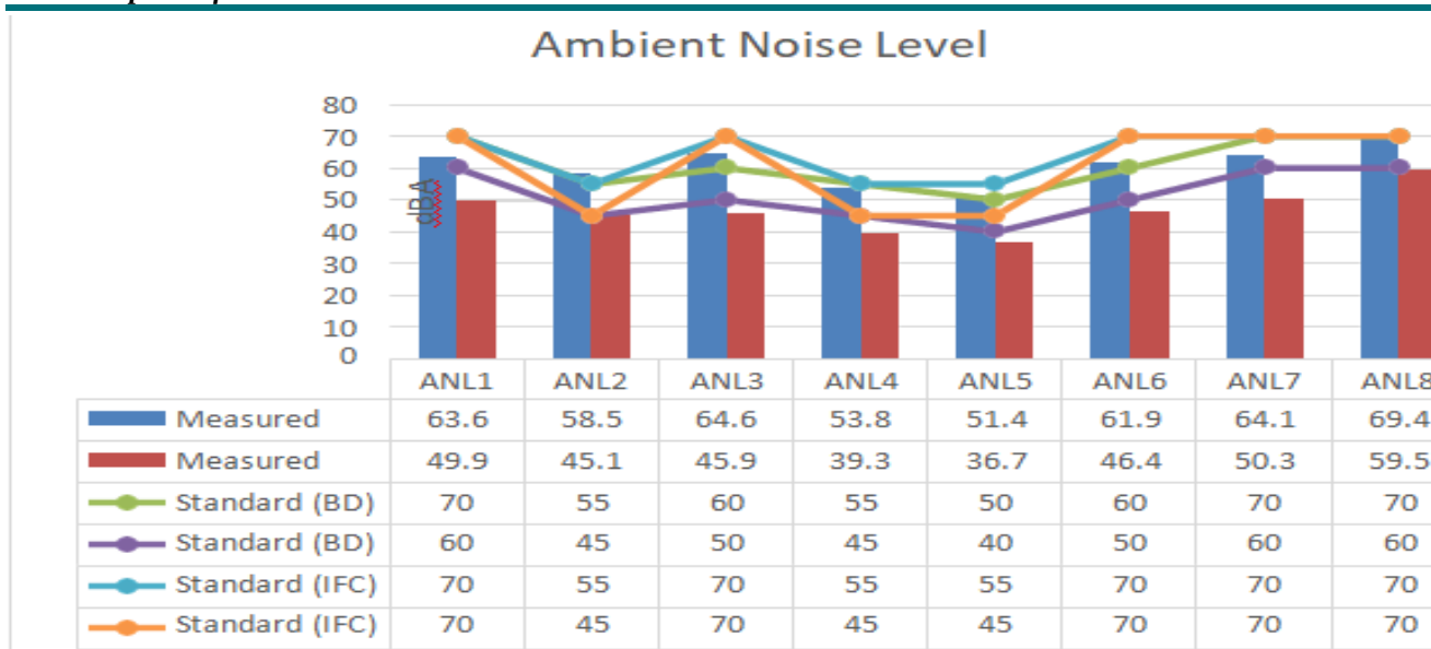
Figure 4-17: Noise Level Results
