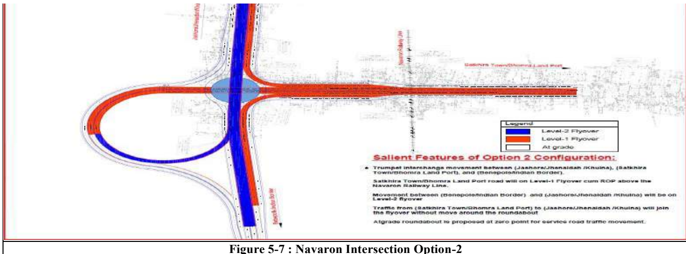
Figure 5-7 : Navaron Intersection Option-2
