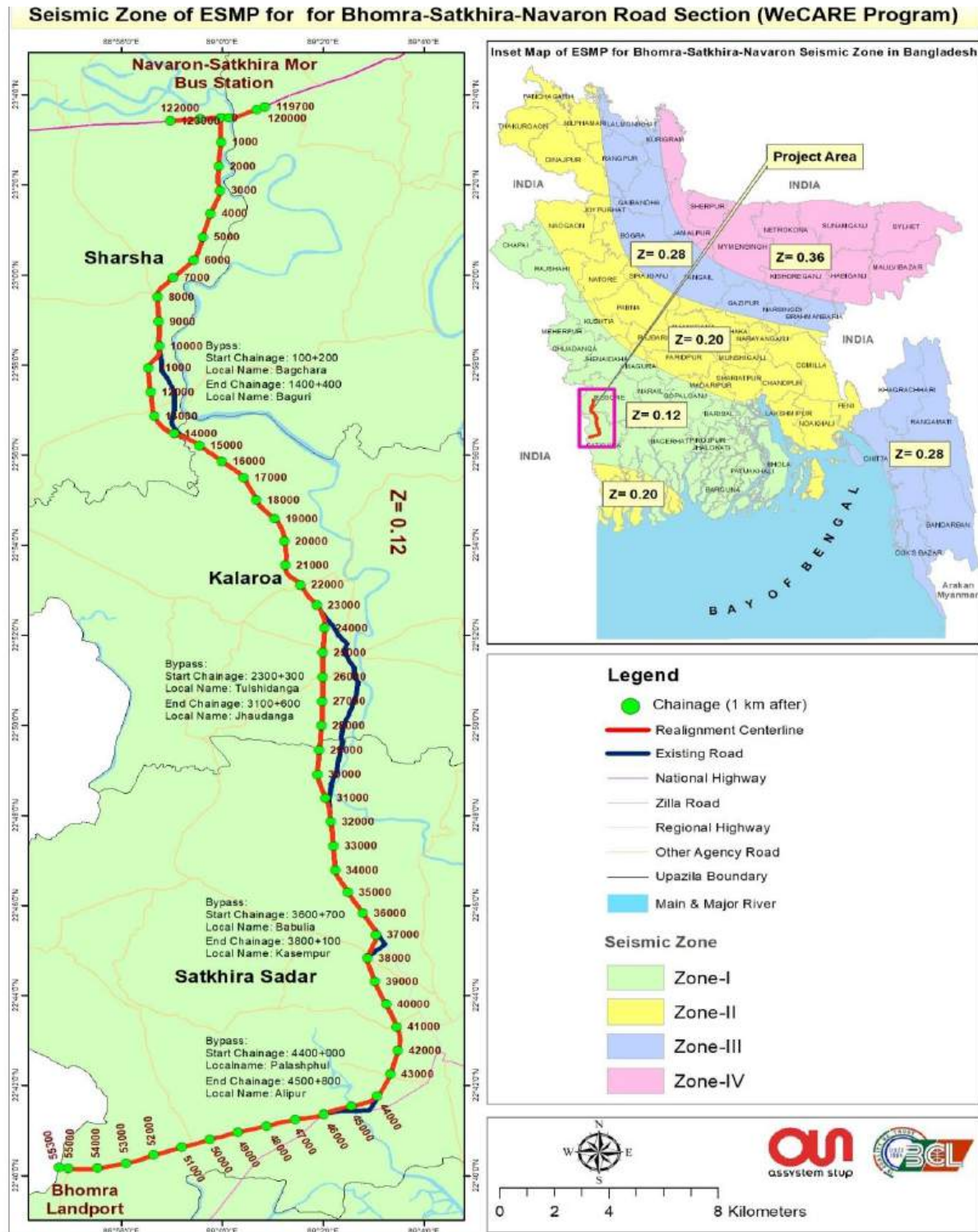
Figure 4-4: Seismic Zoning Map
