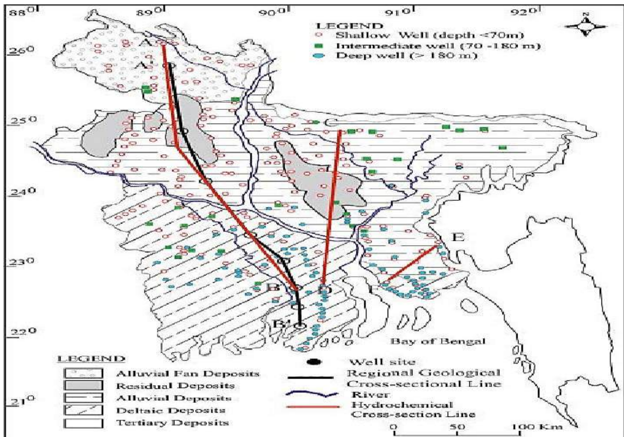
Figure 4-3: Geological Map at Bhomra – Satkhira – Navaron Road
