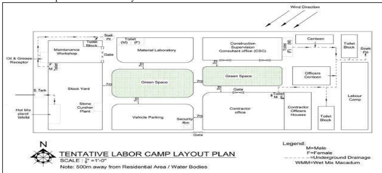
Figure 8-1: Tentative Layout of the Construction/Workers Camp
