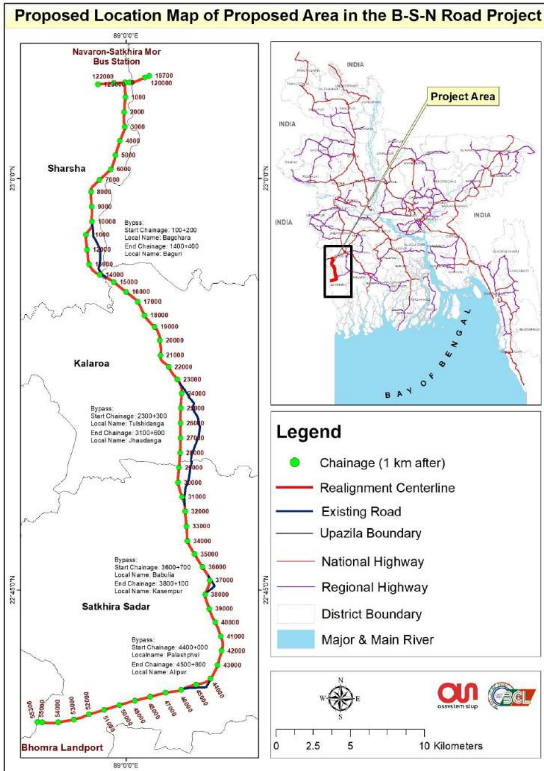
Figure 5-1: Existing and Proposed Realignment for Bagachhra Urban Area
