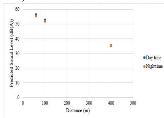
Figure 7-3: Incremental Noise Levels at Different Distances (m)
