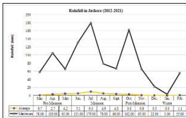
Figure 4-11: Average Rainfall Variation in the Jashore Region from 2012 to 2021
