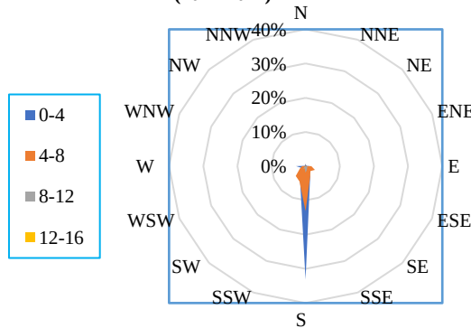
Figure 4-14: Seasonal Variation of Wind Rose in Jashore during the Years of 2012-2021
