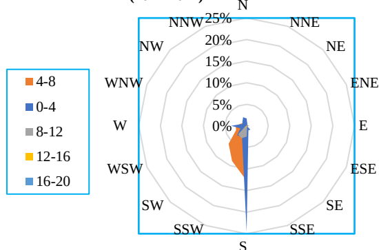
Figure 4-13: Seasonal Variation of Wind Rose in Jashore during the Years of 2012-2021
