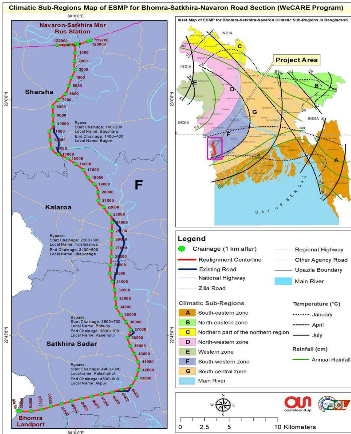
Figure 4-9: Climate Sub-region for Bhomra-Satkhira-Navaron Road Section
