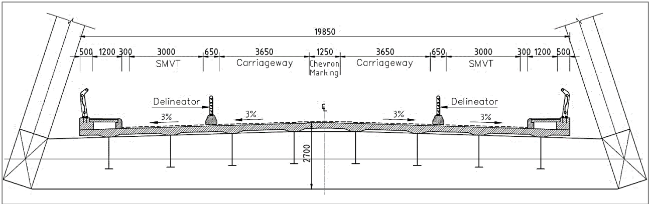
Figure 4-2: Cross Section of Steel Arch bridge
