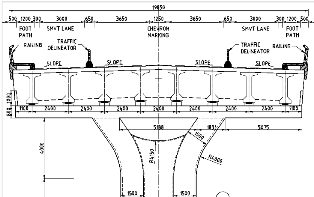
Figure 4-3: Cross Section of PSC I-Girder Type Viaduct
