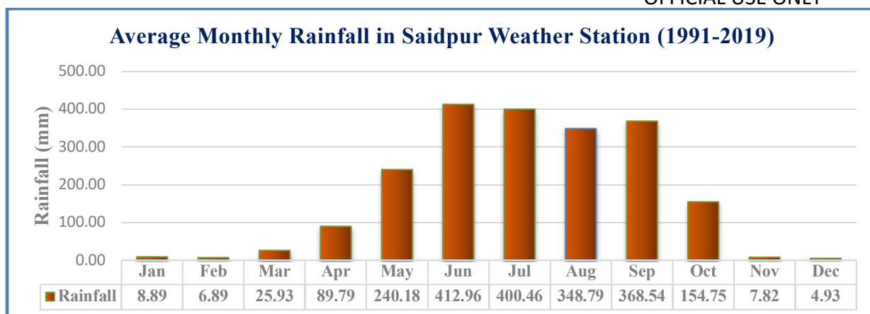
Figure IV.33: Average Monthly Rainfall of Saidpur Weather Station
