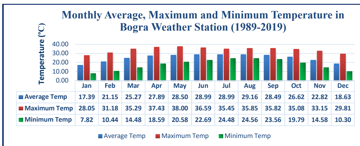
Figure IV.2: Monthly Average, Maximum and Minimum Temperature of Bogra Weather Station
