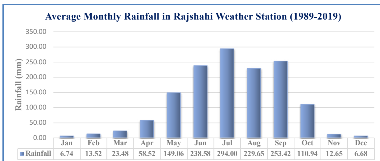
Figure IV.7: Average Monthly Rainfall of Rajshahi Weather Station
