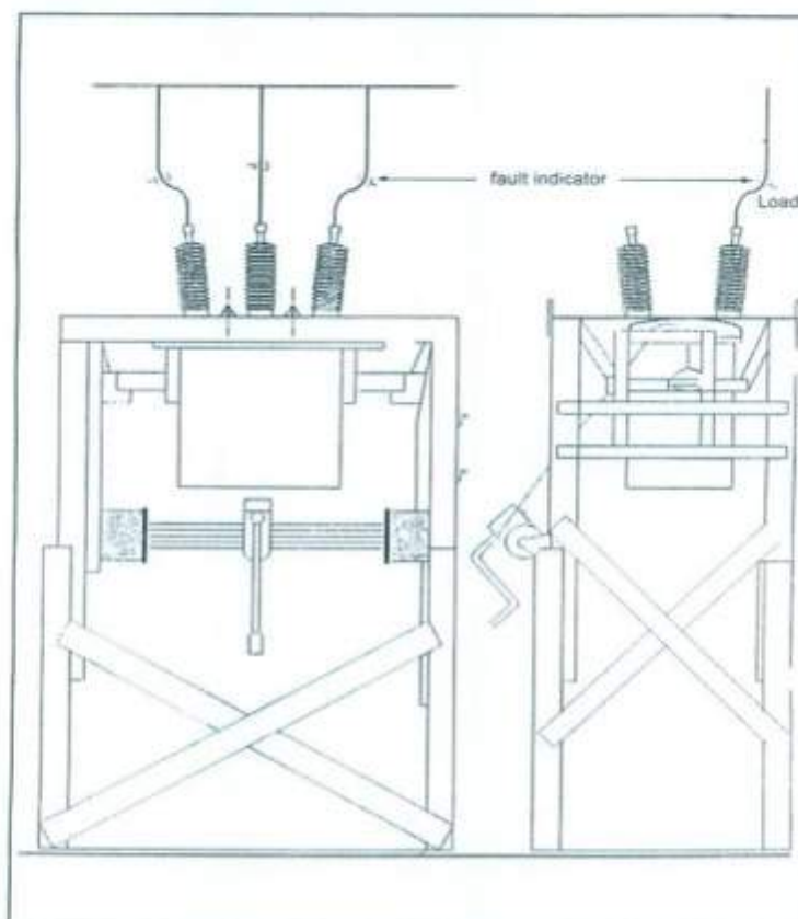
Figure 5-2: Location of fixing Fault Indicator
