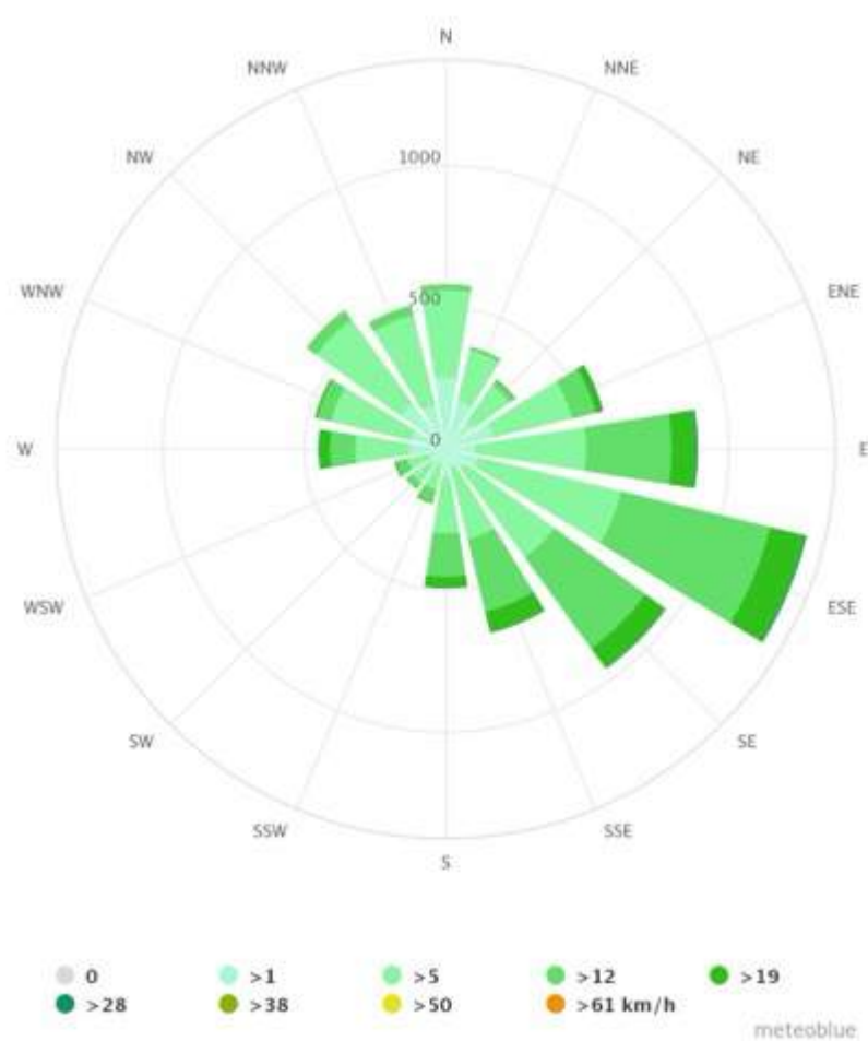
Figure IV.11: Wind rose diagram of Ishwardi Weather Station
