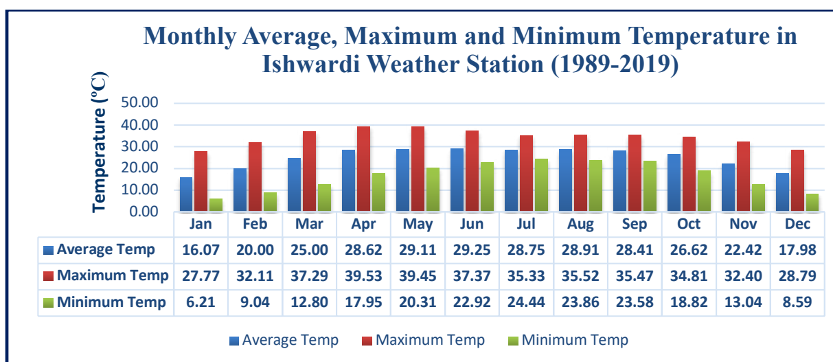
Figure IV.3: Monthly Average, Maximum and Minimum Temperature of Ishwardi Weather Station
