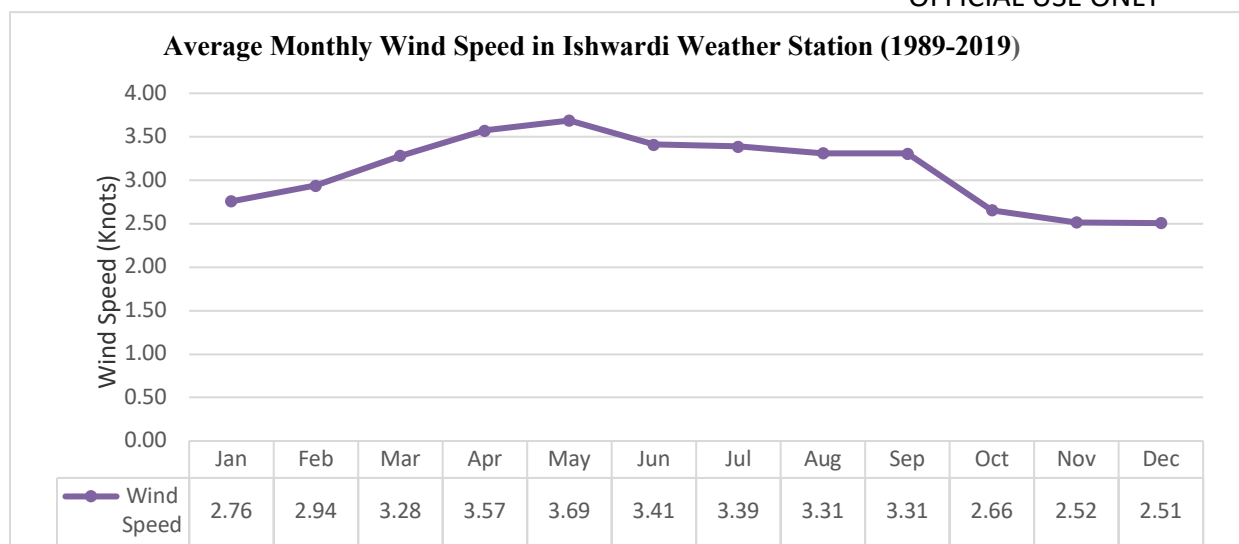
Figure IV.10: Average Monthly Wind Speed of Ishwardi Weather Station
