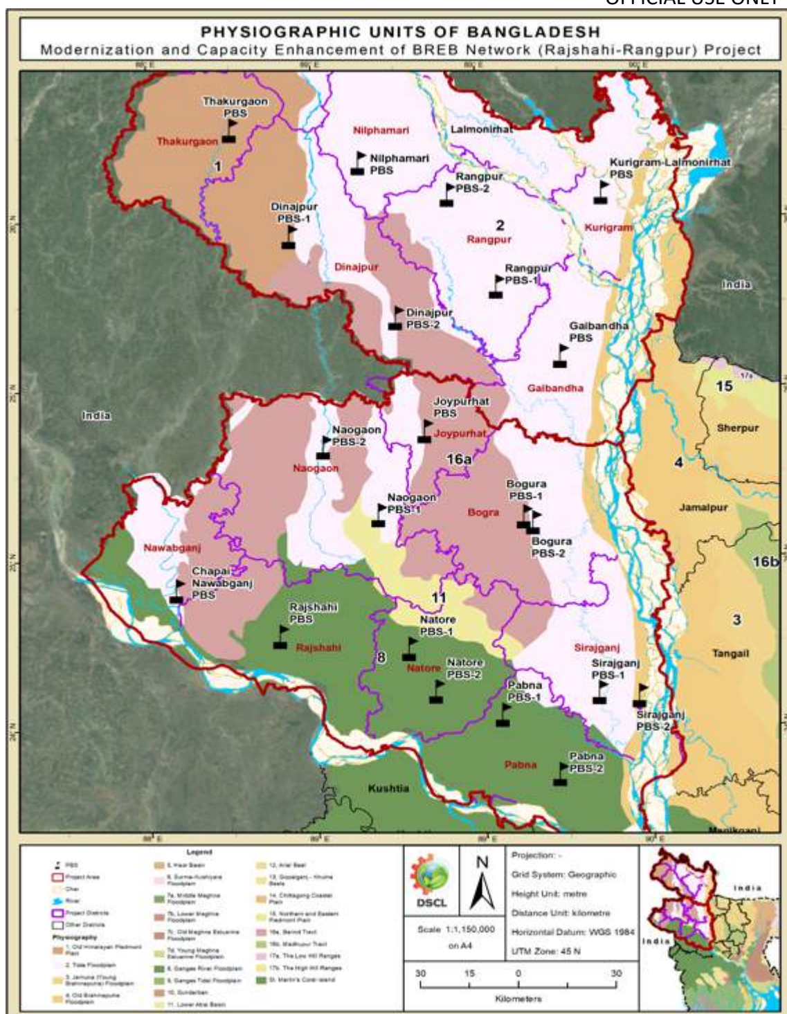
Figure IV.17: Physiographic map of study area
