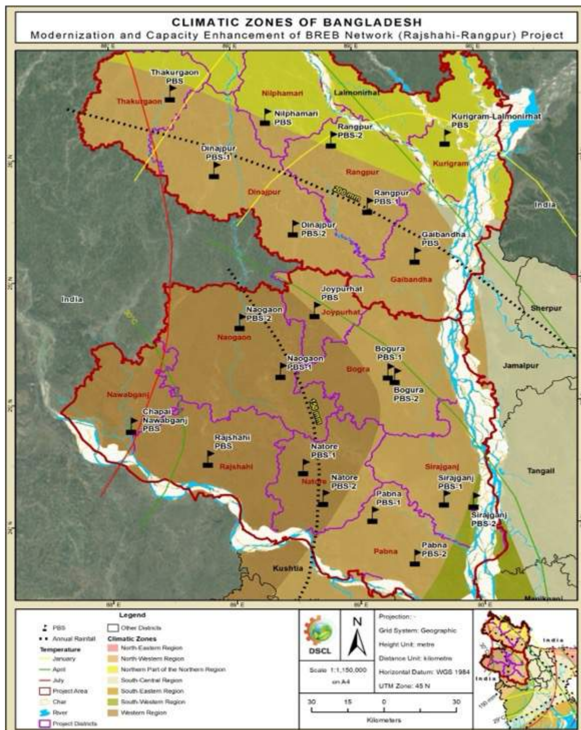
Figure IV.1: Climate Zone of study area
