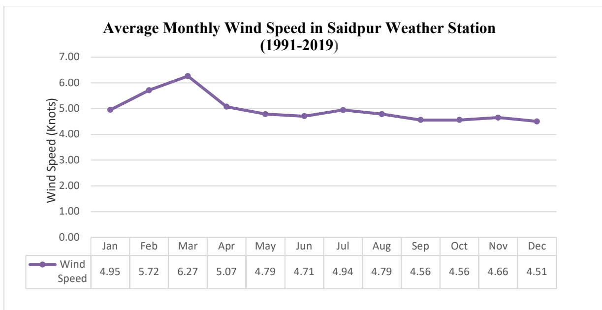
Figure IV.38: Average Monthly Wind Speed of Saidpur Weather Station
