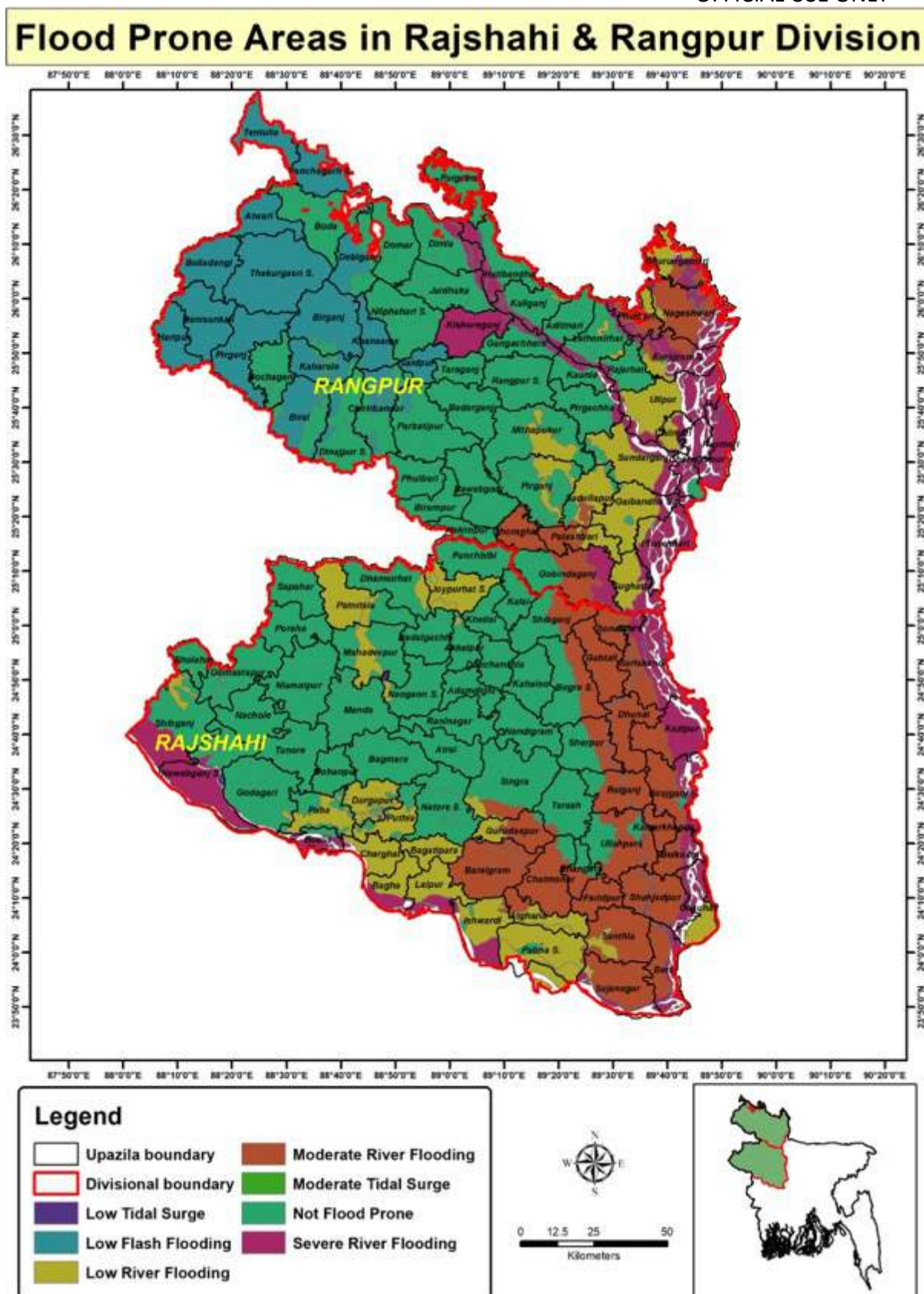
Figure III.13: Flood Prone area map under Rajshai-Rangpur division.
