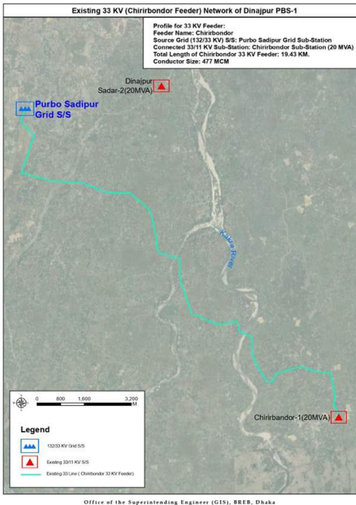
Figure III.4: Existing 33 kv distribution network of Dinajpur PBS-01
