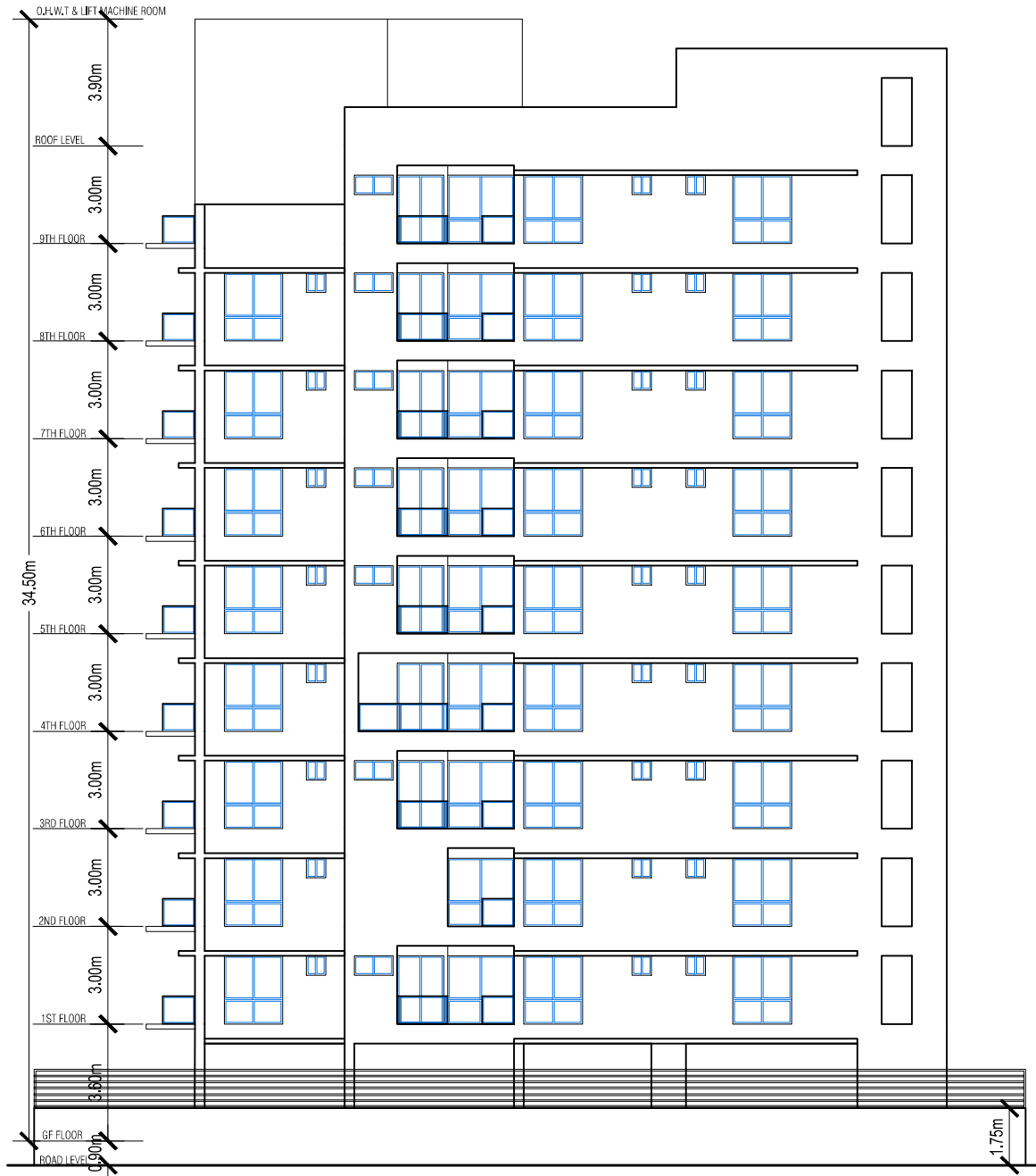
EAST ELEVATION
