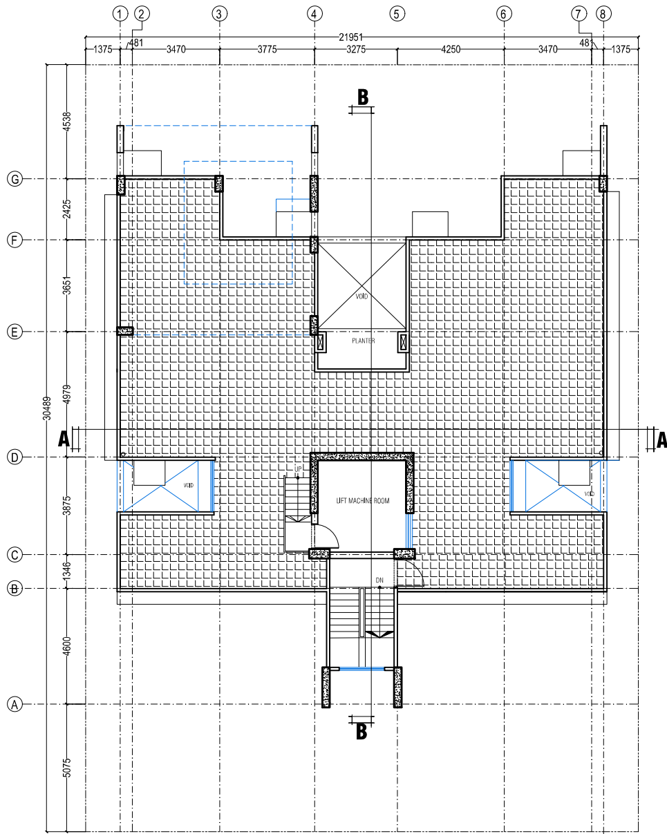
ROOF SCALE -1:100
