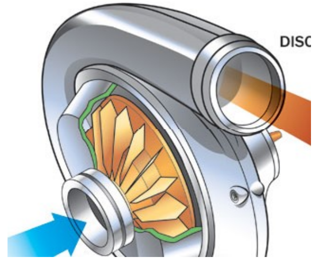
How Superchargers Work
