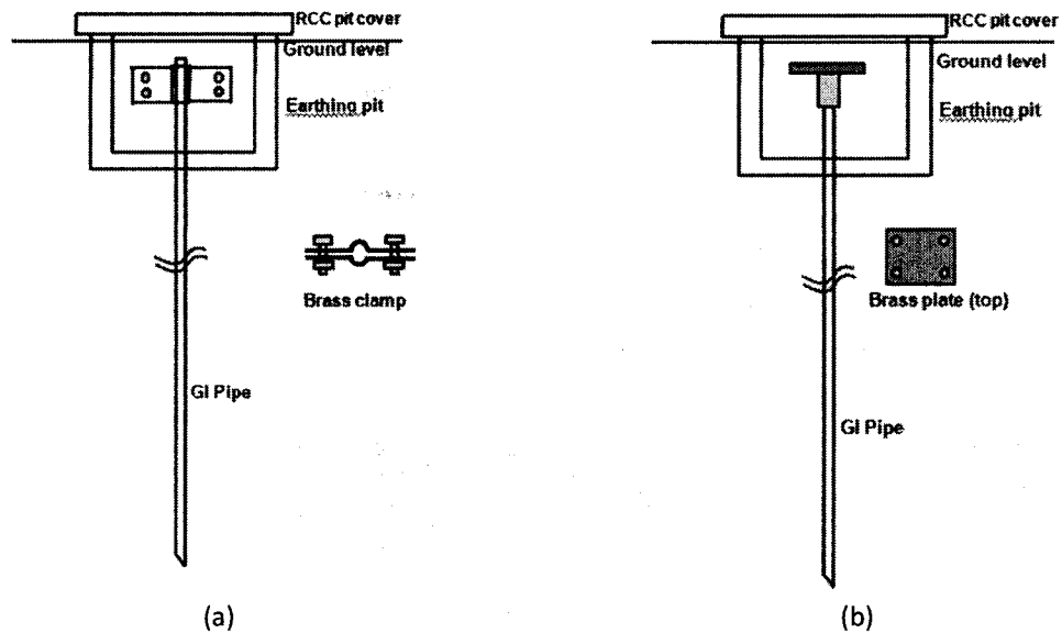
Figure 3 Pipe Earthing; (a) Type 1; (b) Type 2
