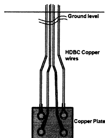
Figure 2 Copper Plate Earthing
