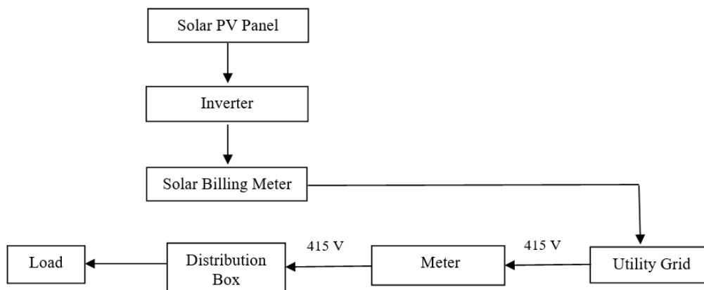
Figure 04: Metering Diagram for Direct Power Evacuation
