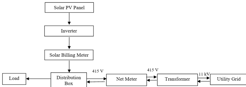
Figure 03: Metering Diagram for LTCT Customer
