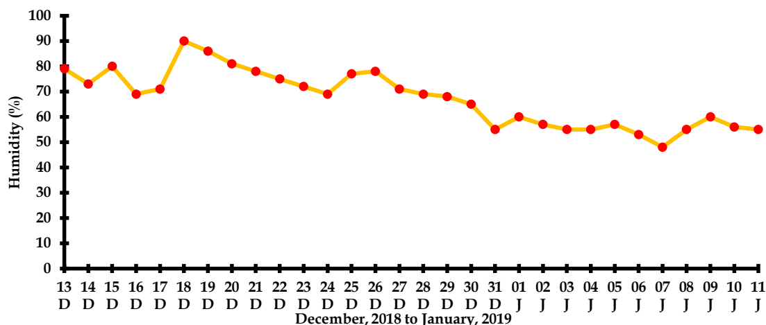
Fig. 11. Air humidity during seedling growing period
