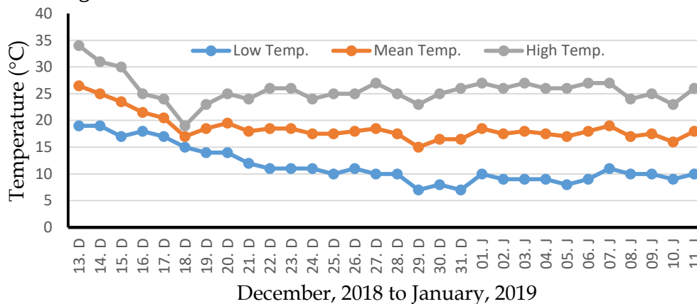
Fig. 80. Ambient temperature during study period (December 2018 to January 2019)
