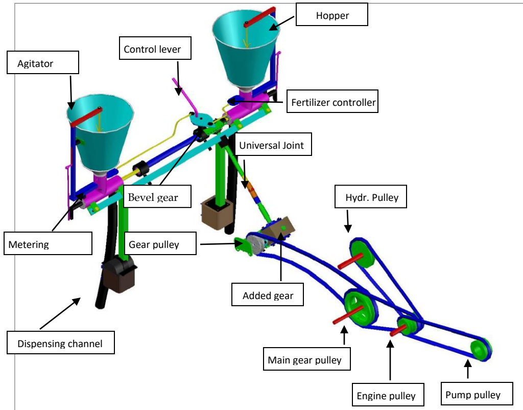
Fig. 29. Power transmission from engine to the mixed fertilizer applicator
