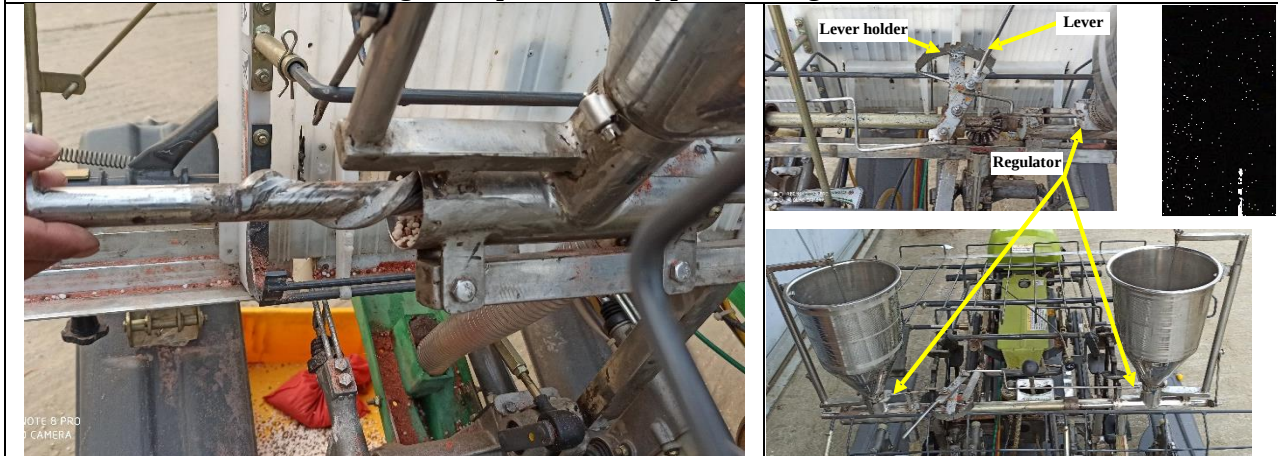
Fig. 39. Spiral screw attached in the metering chamber
