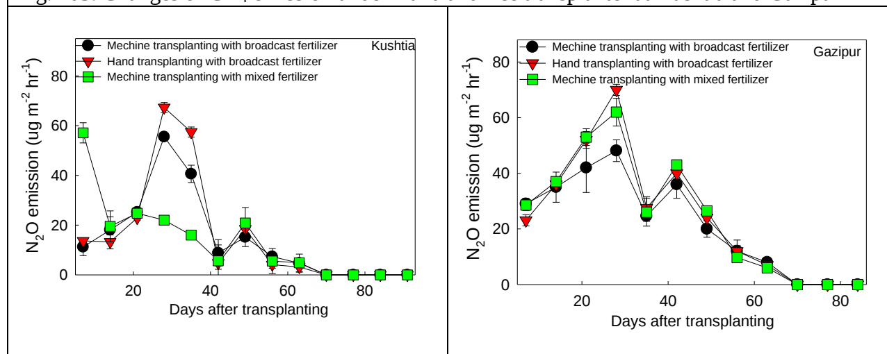
Fig. 104. Changes of \text{N}_2\text{O} emission under Hand and rice transplanter at Kushtia and Gazipur
