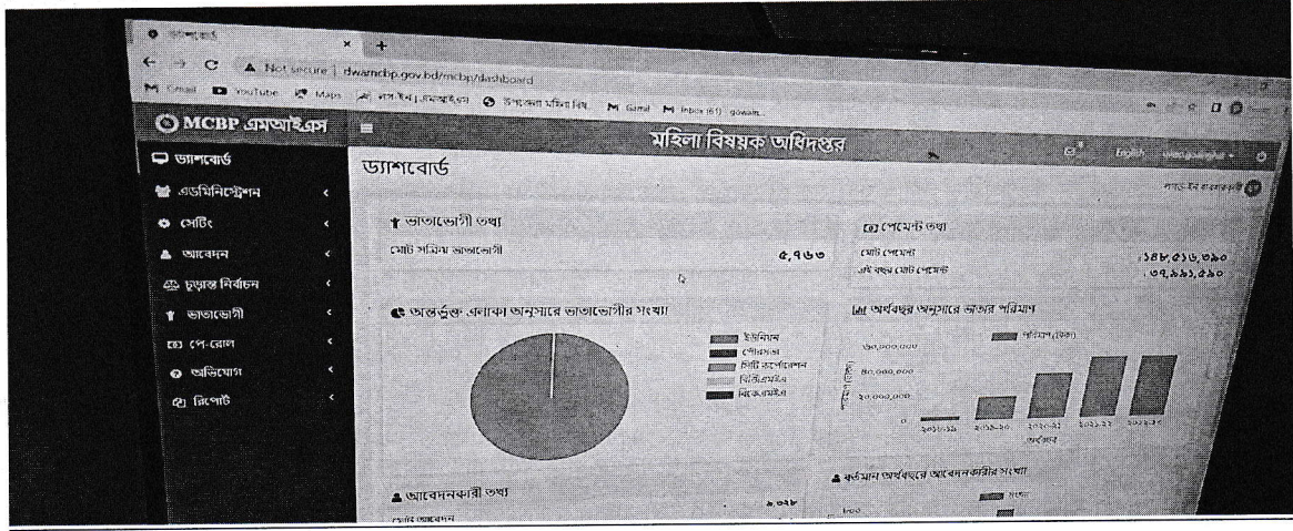
MCBP Software
