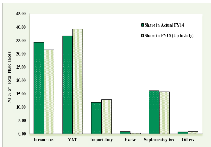
FIGURE 7: SHARE AMONG NBR TAXES
