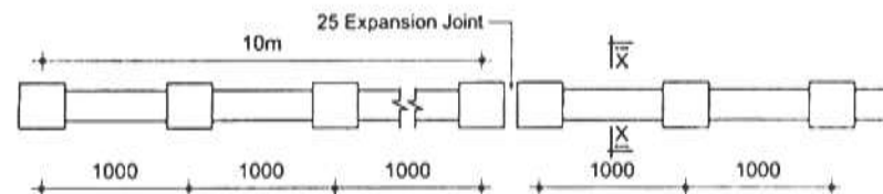
Plan of RCC Post & Wall
