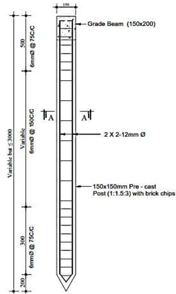
Reinf. Details of RCC Post
