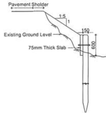
RCC PALISADING
