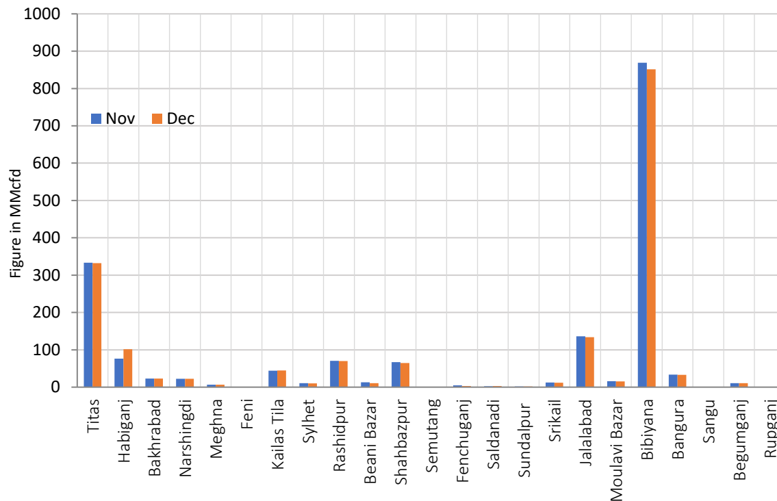
Figure 8: Comparison of field-wise daily avg. Gas production between November 2025 & December 2025
