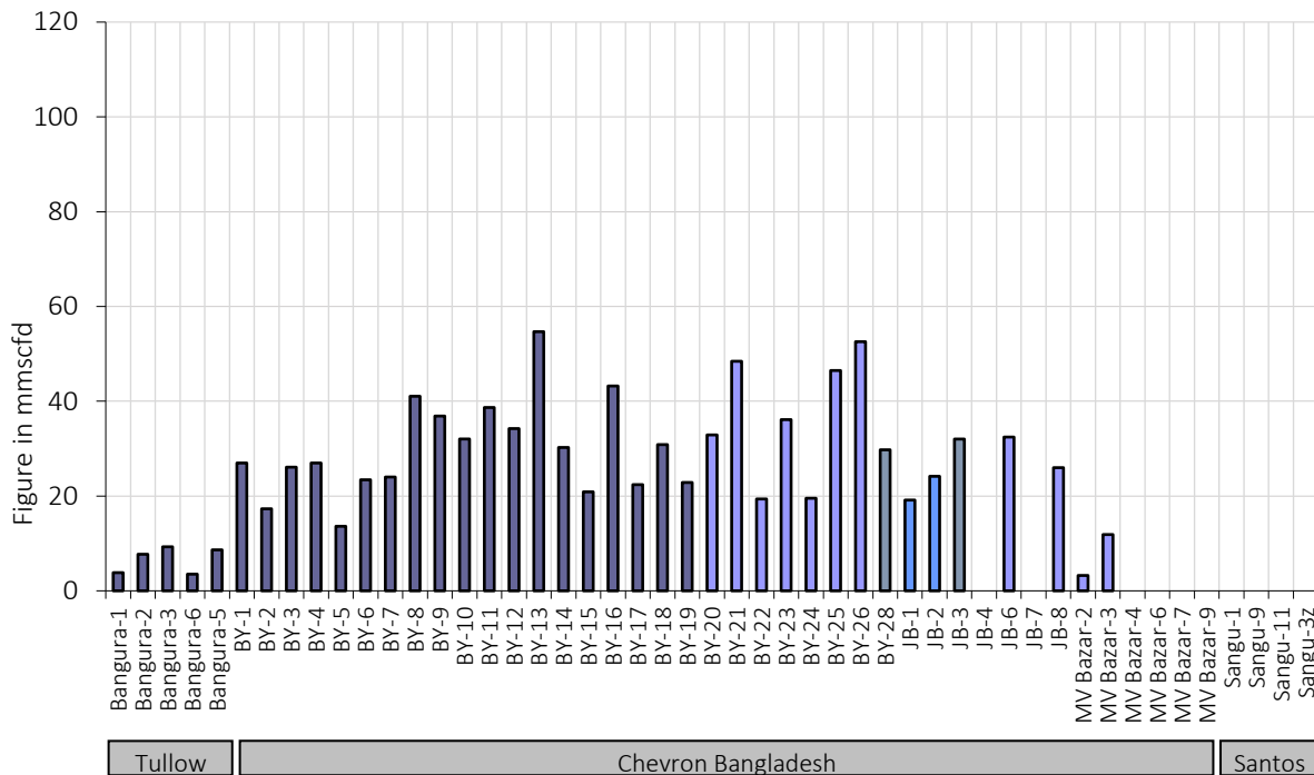
Figure 7: Well-wise Daily Average Production- IOC and JVA December 2025
