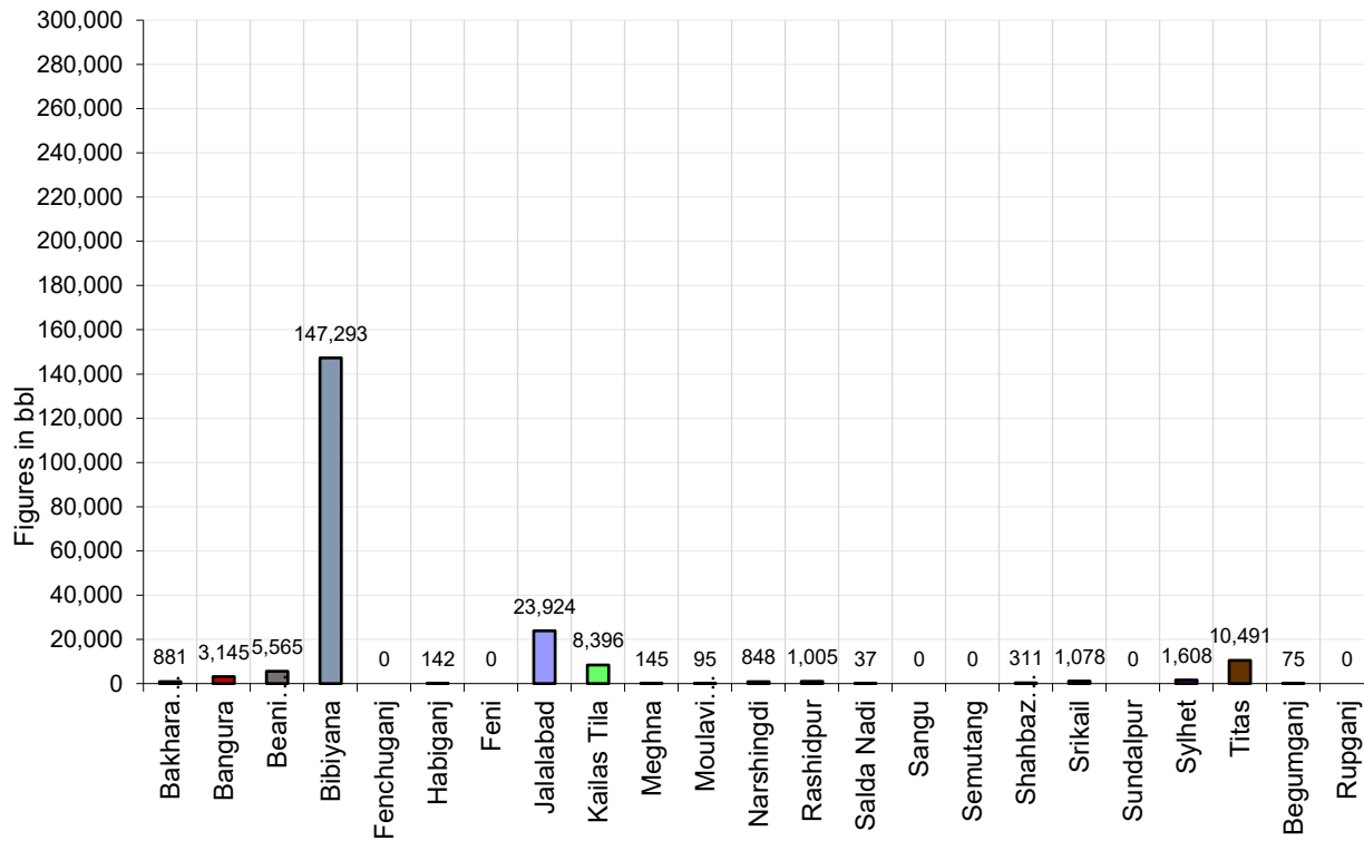
Figure 14: Monthly Condensate Production December 2025
