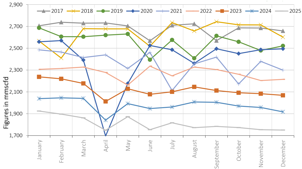
Figure 3: Daily Average Production (from January 2017 to December 2025 ) replenishment, improved production management, and alternative energy sourcing.
