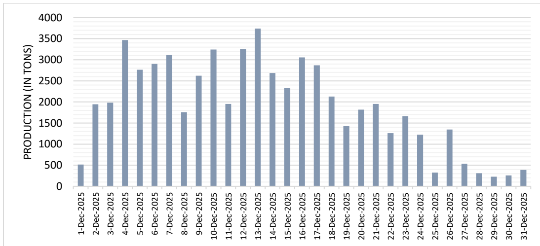
Figure 15: Barapukuria Coal Mine Daywise Data Graph for December 2025
