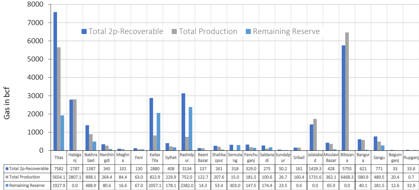
Figure 2: Reserve, Production and Remaining Reserve as of December 2025
