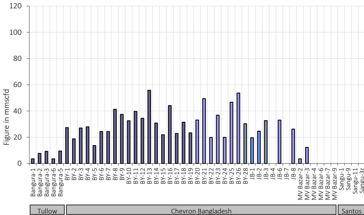
Figure 7: Well-wise Daily Average Production- IOC and JVA November 2025
