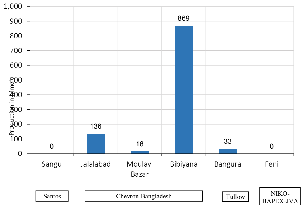
Figure 13: Daily Avg. Production - IOC and JVA November 2025
