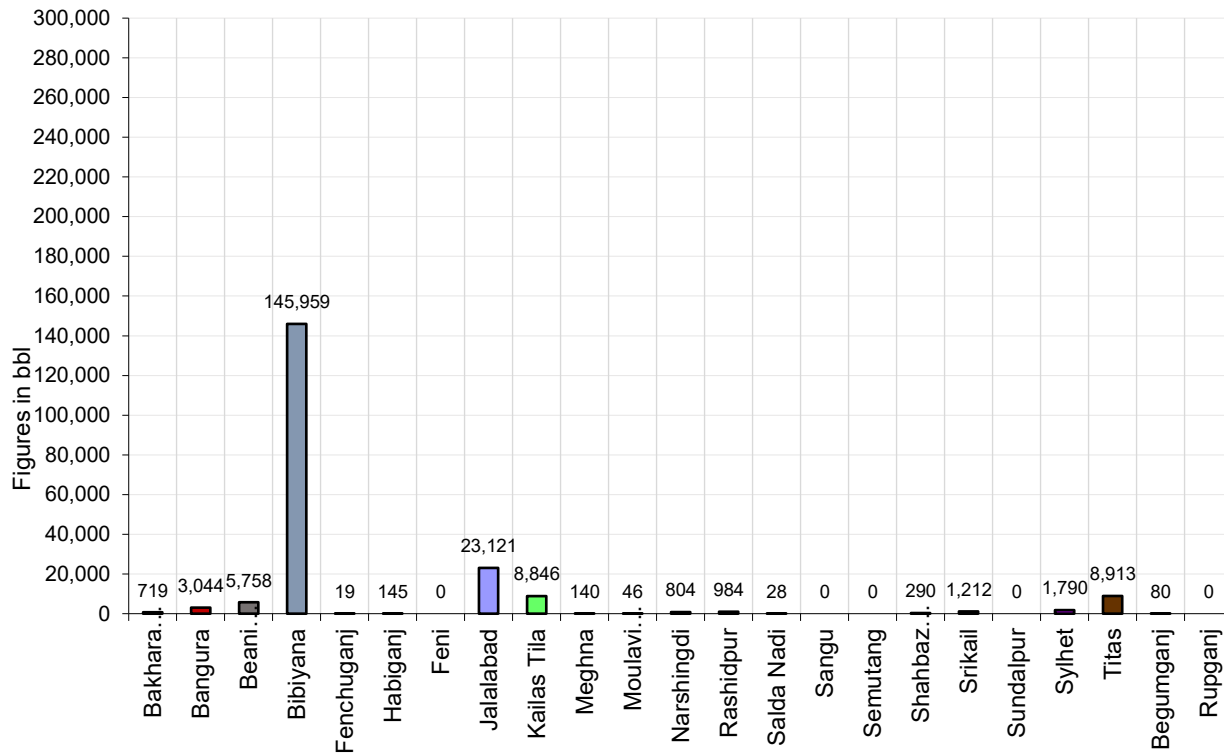
Figure 14: Monthly Condensate Production November 2025
