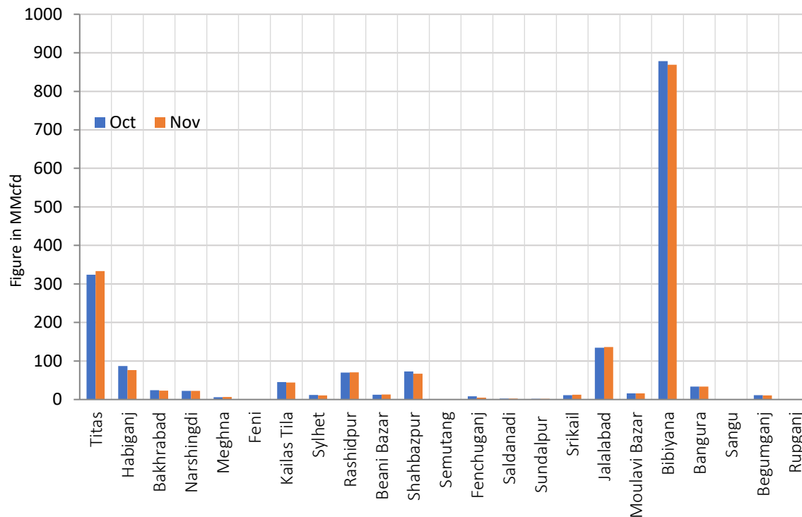
Figure 8: Comparison of field-wise daily avg. Gas production between October 2025 & November 2025
