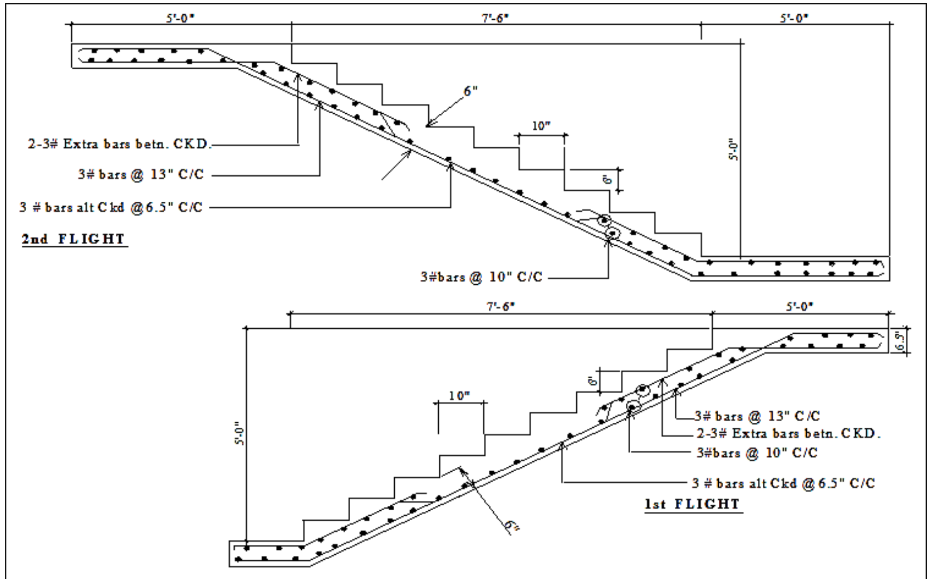
REINFORCEMENT DETAILING OF STAIR
