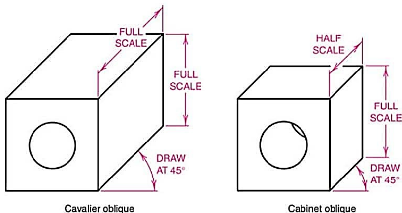
Figure: Oblique drawing
