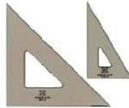
2. Triangles
