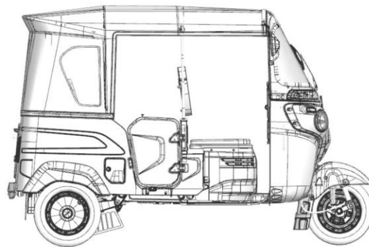
RIGHT HAND SIDE VIEW
