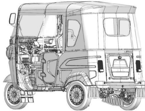
LEFT REAR PERSPECTIVE VIEW
