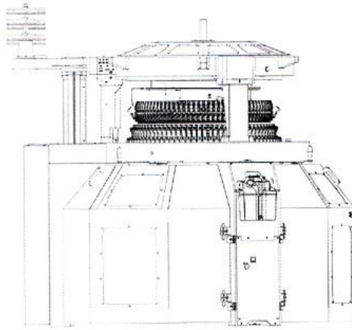
View: Left View
