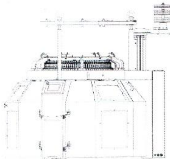
View: Front View
