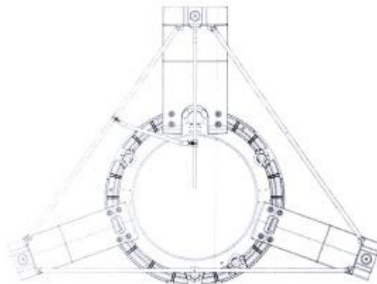
View: Top View
