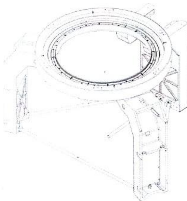
View: Perspective View
