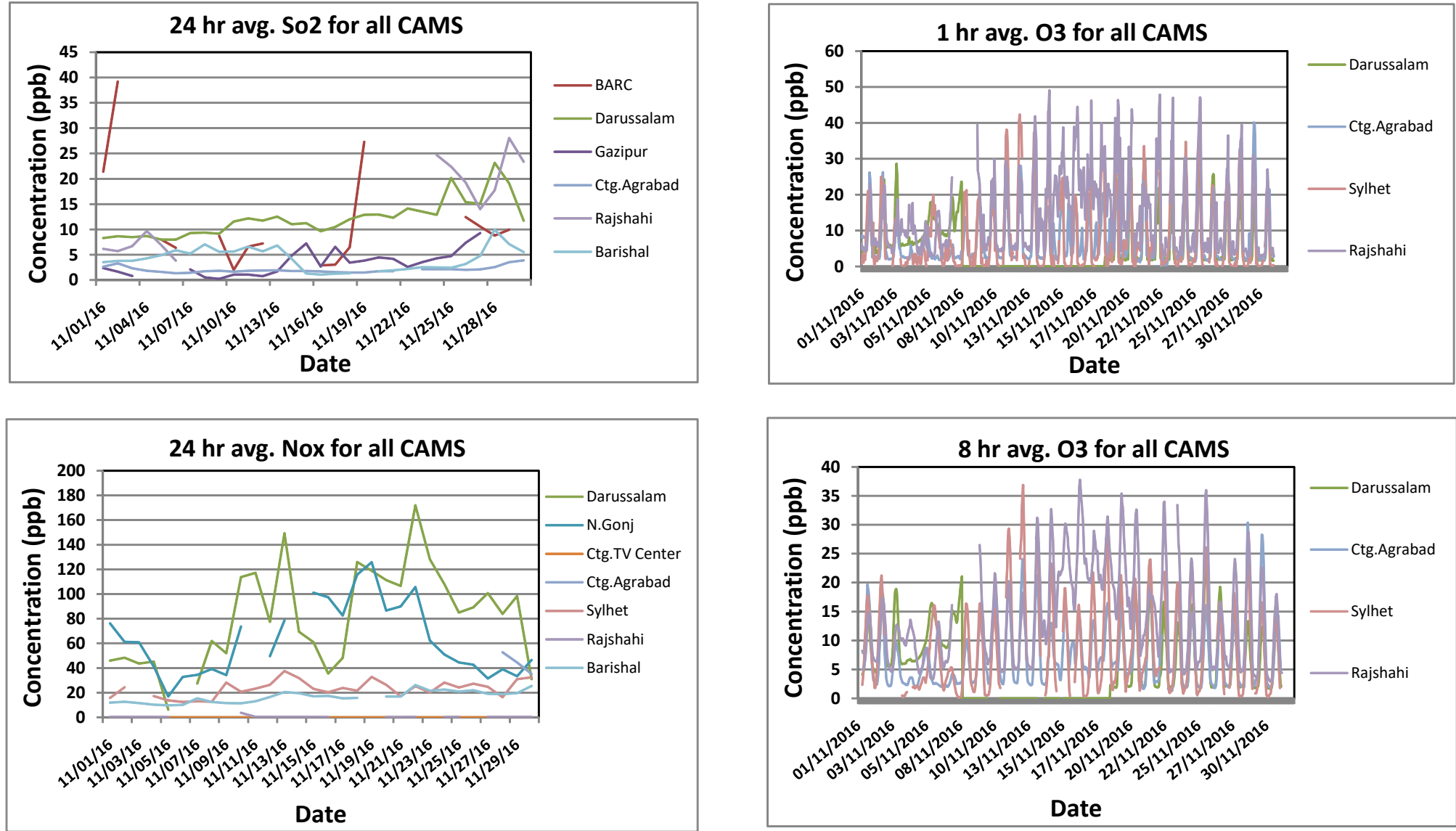
FIGURE 3: TIME SERIES OF ALL PARAMETERS (SO 2 , NO x AND O 3 ) MEASURED IN ALL CAMS DURING NOVEMBER, 2016
