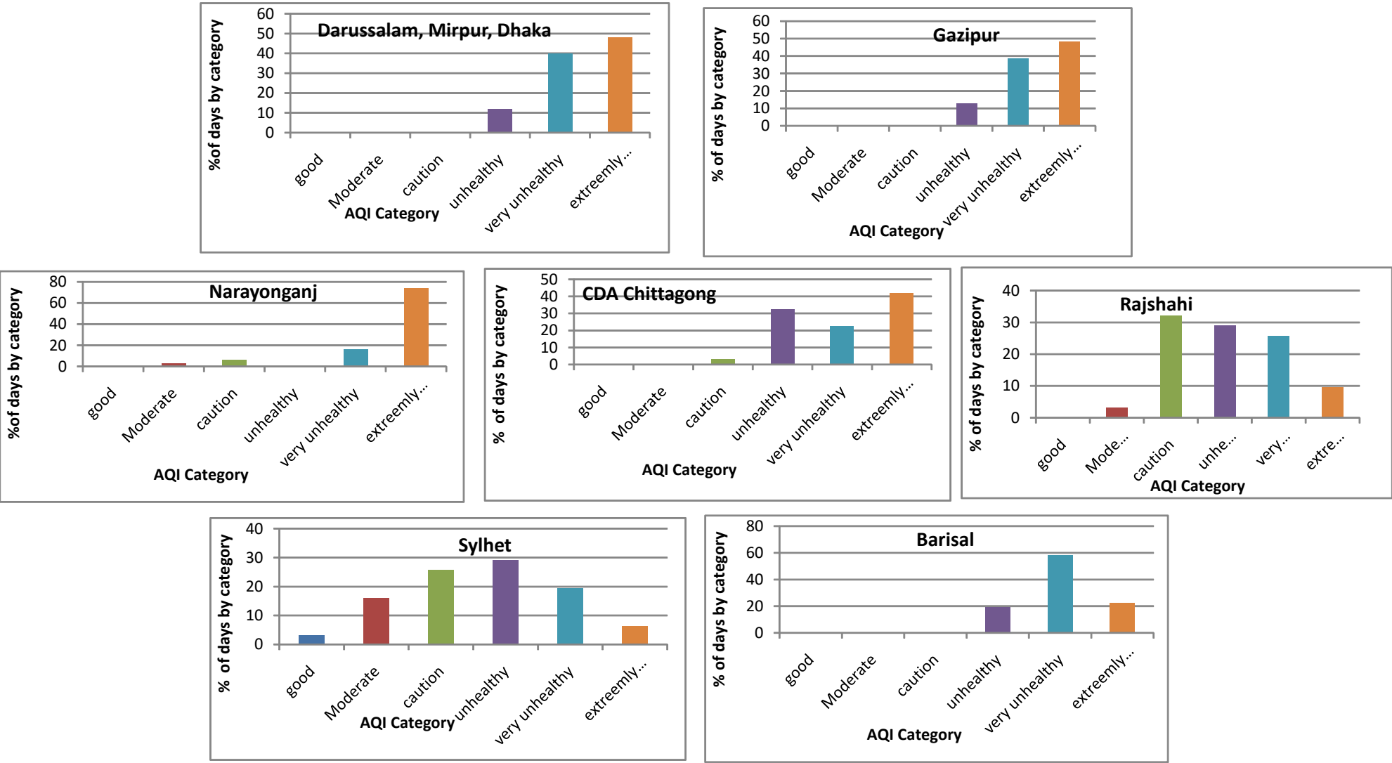
Figure 5: Monthly Summary of AQI for month of December, 2016
