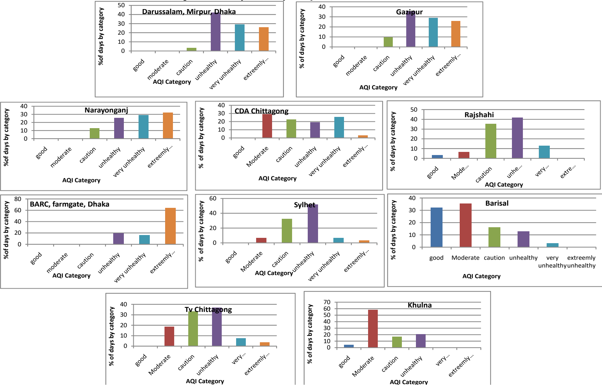
Figure 5: Monthly Summary of AQI for month of March, 2018
