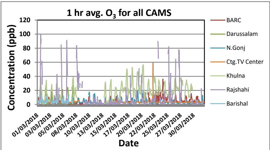
FIGURE 3: TIME SERIES OF ALL PARAMETERS (SO 2 , NO x AND O 3 ) MEASURED IN ALL CAMS DURING MARCH, 2018
