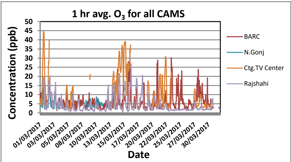
FIGURE 3: TIME SERIES OF ALL PARAMETERS (SO 2 , NO x AND O 3 ) MEASURED IN ALL CAMS DURING MARCH, 2017
