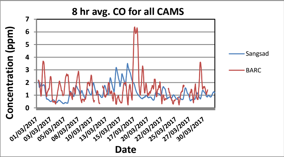
Figure 4: TIME SERIES OF ALL PARAMETERS (CO, PM10 AND PM2.5) MEASURED IN CAMS DURING MARCH, 2017
