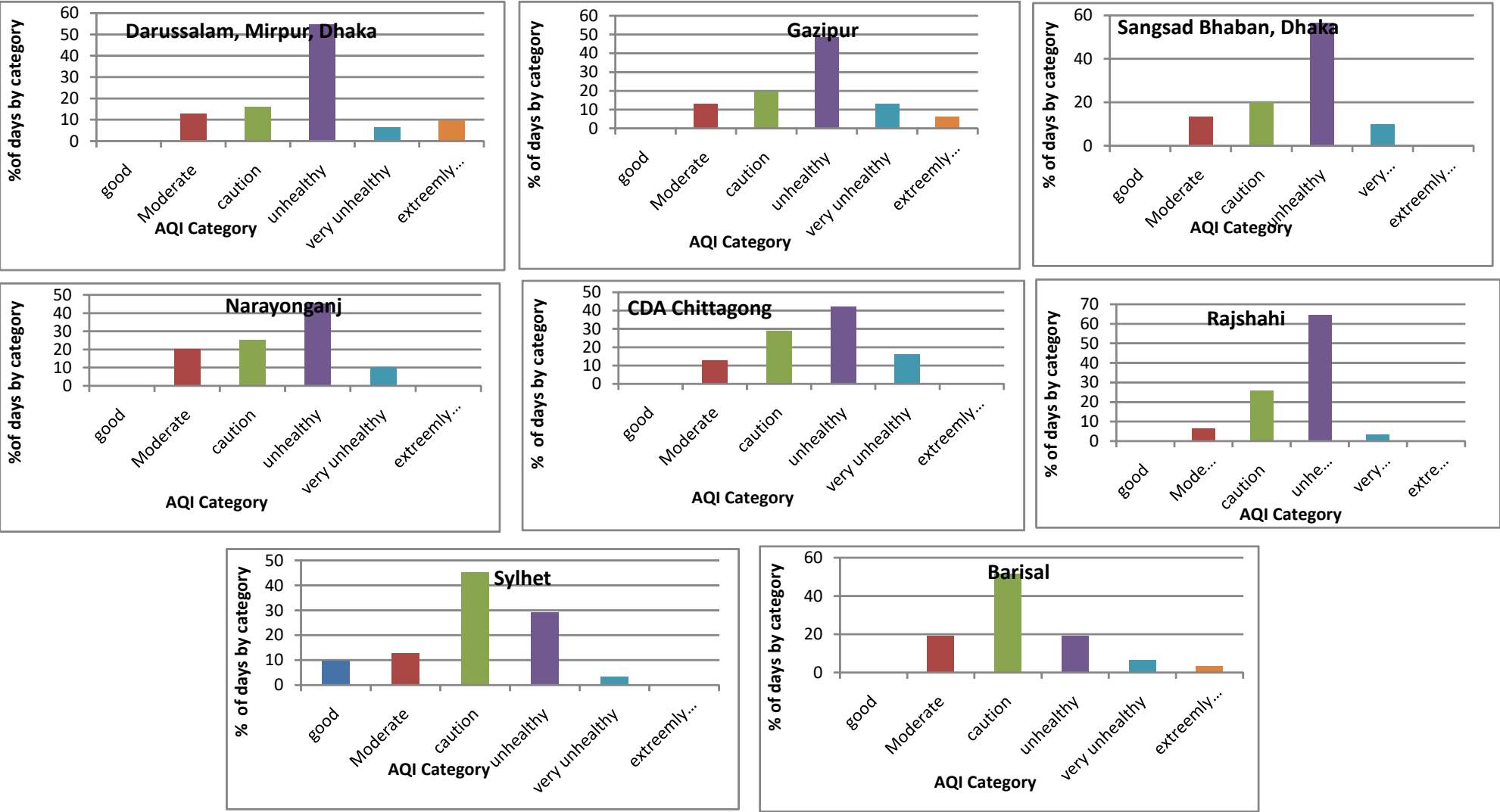
Figure 5: Monthly Summary of AQI for month of March, 2017
