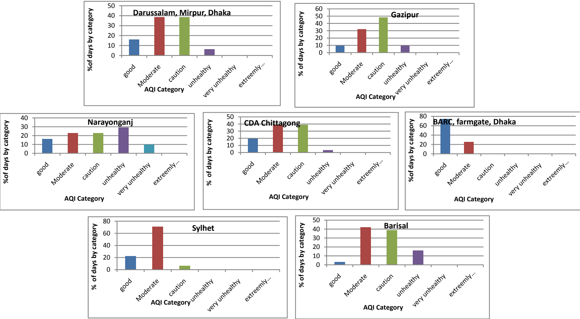
Figure 5: Monthly Summary of AQI for month of October, 2016
