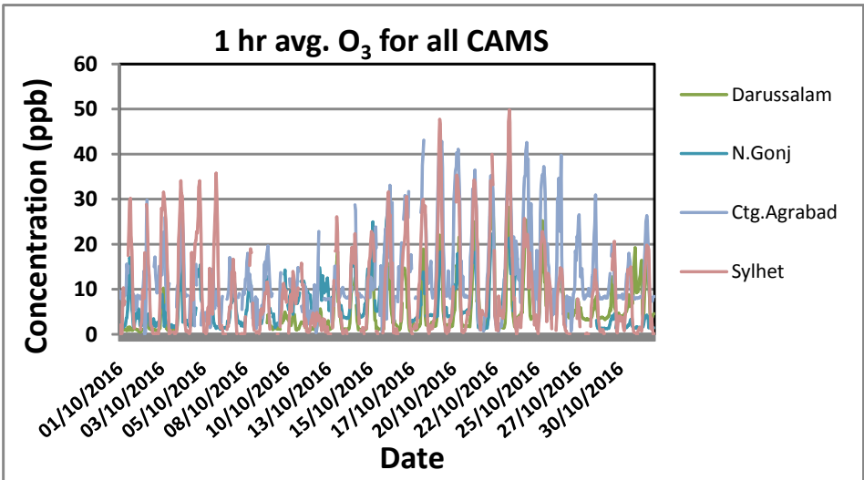
FIGURE 3: TIME SERIES OF ALL PARAMETERS (SO 2 , NO x AND O 3 ) MEASURED IN ALL CAMS DURING OCTOBER, 2016
