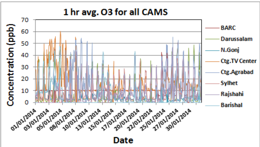
TIME SERIES OF ALL PARAMETERS (SO 2 , NO x AND O 3 ) MEASURED IN ALL CAMS DURING January 2014
