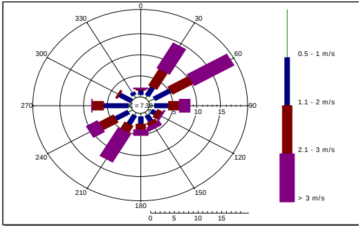
Wind Rose of BARC CAMS
