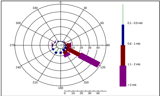
Wind Rose of Sangsad CAMS
