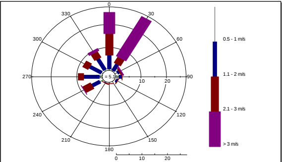
Wind Rose of Barisal CAMS
