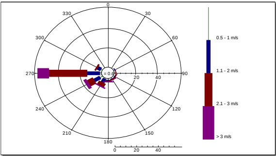
Wind Rose of Darussalam CAMS
