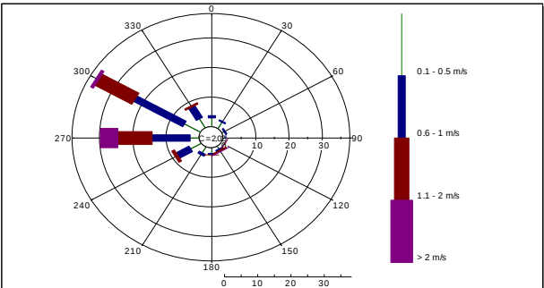
Wind Rose of Sangsad CAMS
