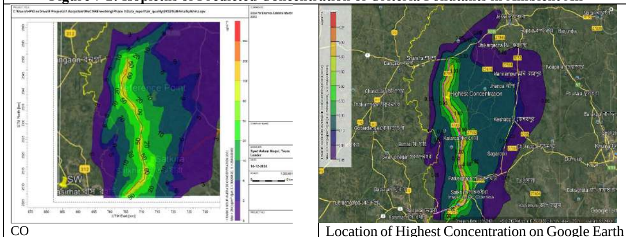
Figure 7-2: Isoleths of Predicted Concentration of Criteria Pollutants in Ambient Air
