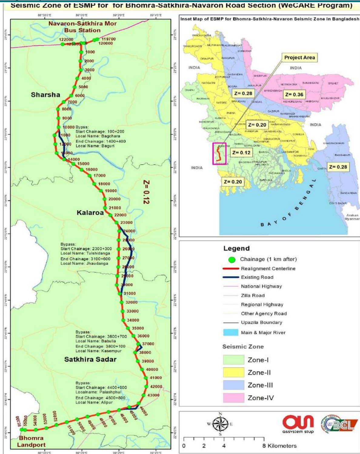
Figure 4-3: Seismic Zoning Map
