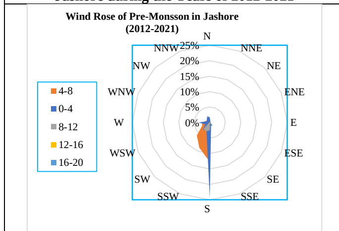
Figure 4-12: Seasonal Variation of Wind Rose in Jashore during the Years of 2012-2021
