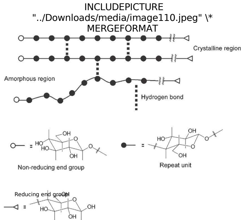
17.3 Schematic representation of cellulose fibre internal structure.
