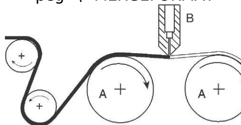
2.3 Machnozzle system. Reprinted from Textiles Sciences and Technology 11: Textile processing and properties: preparation, dyeing, finishing and performance , T.L. Vigo (ed.), 1997, Chap 4, p 275, with permission from Elsevier.
