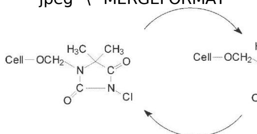
Treatment with OCl converts back to 15.4 Renewable
