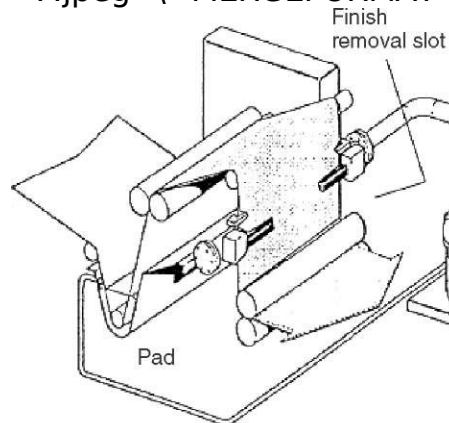
2.2 Vacuum extraction system. Rep Finishing: a technical guide , 1997, p 157, courtesy of Cotton Incorporated, Cary, NC.
