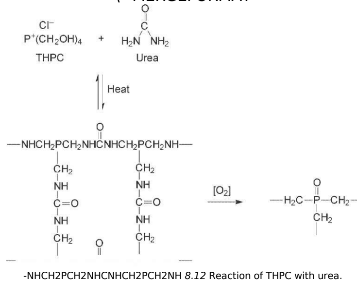
8.12 Reaction of THPC with urea.
