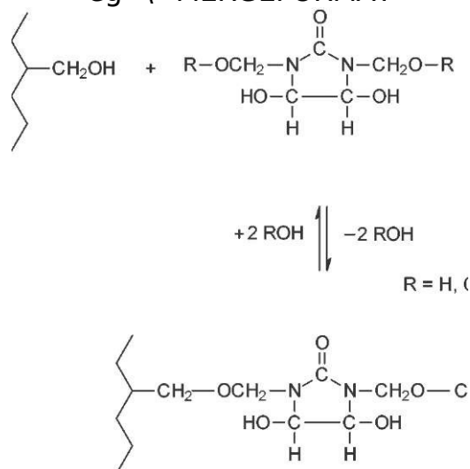
5.5 Crosslinking of cellulose with DMDHEU products.
