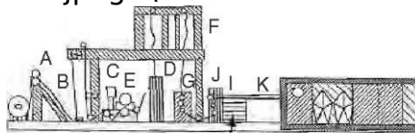
2.13 Tenter frame. Reproduced from Cotton Dyeing and Finishing: a technical guide , 1997, p 166, courtesy of Cotton Incorporated, Cary, NC.
