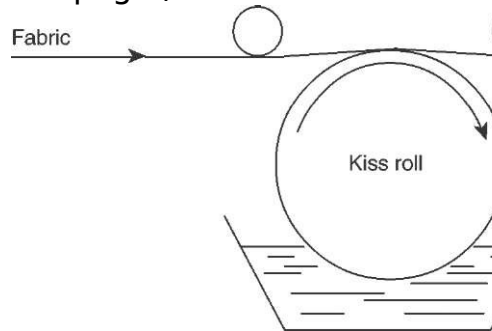
2.4 Kiss roll applicator. Reproduced from Cotton Dyeing and Finishing: a technical guide , 1997, p 153, courtesy of Cotton Incorporated, Cary, NC.
