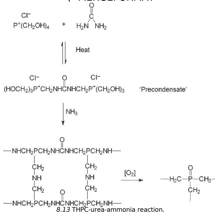
8.13 THPC-urea-ammonia reaction.
