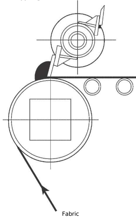
Fabric 2.16 Knife over roll coater. Reproduced from Textile Finishing , D. Heywood (ed.). Bradford, SDC, 2003, by permission of The Society of Dyers and Colourists.
