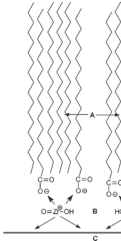
6.1 Fatty acid metal salts. A, hydrophobic interactions; B, polar interactions; C, fibre surface.
