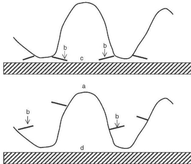
3.7 Schematic arrangement of amino-modified silicone softeners on the fibre surface as suggested by Bereck et al. 13 a = loops of the polydimethylsiloxane chain, b = partially cationic aminoethyl- aminopropyl side groups (about half of them are positively charged), c = fibre surface with partially negative charge, for example cotton and wool, d = hydrophobic attraction of unmodified silicone chain segments and fibre surface, for example polyester.
