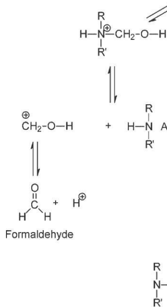
Self c 5.9 W-Methylol reaction scheme.
