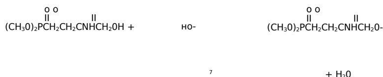
8.14 Reaction of W-methylol dimethylphosphonopropionamide with cellulose.
