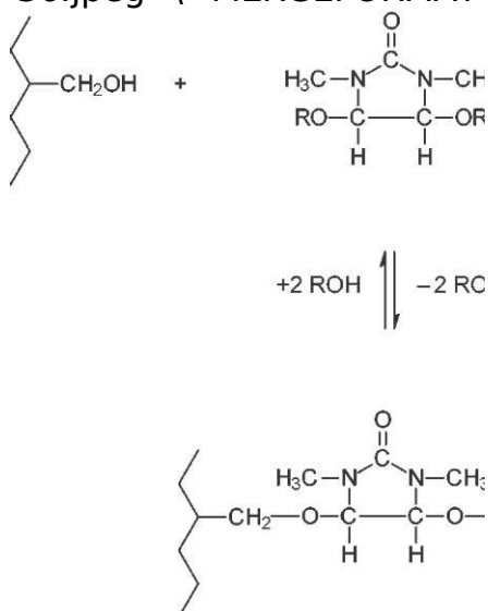
5.7 Crosslinking of cellulose with DMedHEU.
