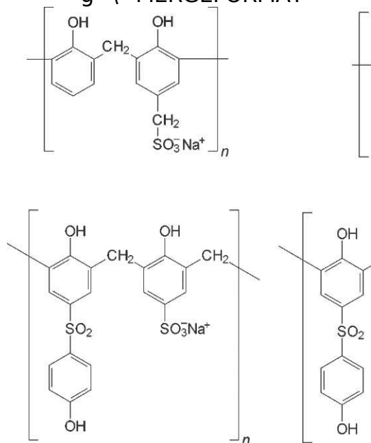
13.3 Reaction products of formaldehyde and aromatic sulfonic acids (syntans) improve wet fastness on nylon.
