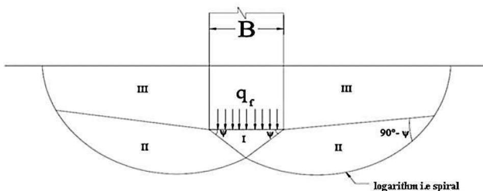
Fig 3.2: Failure zones assumed in Meyerhof's theory
