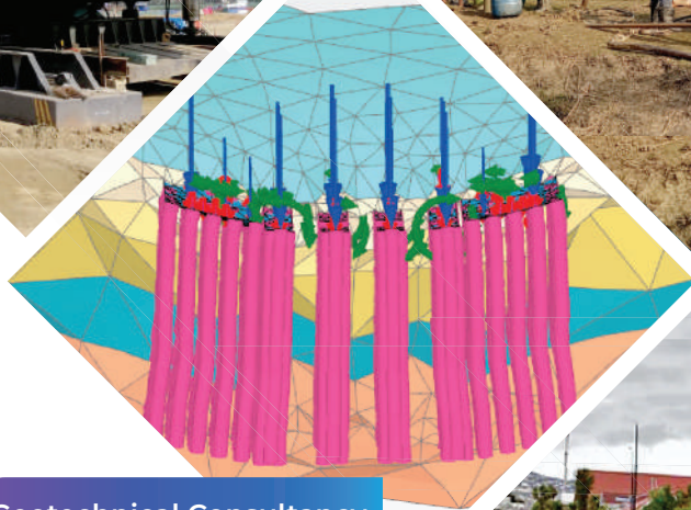
Geotechnical Consultancy
