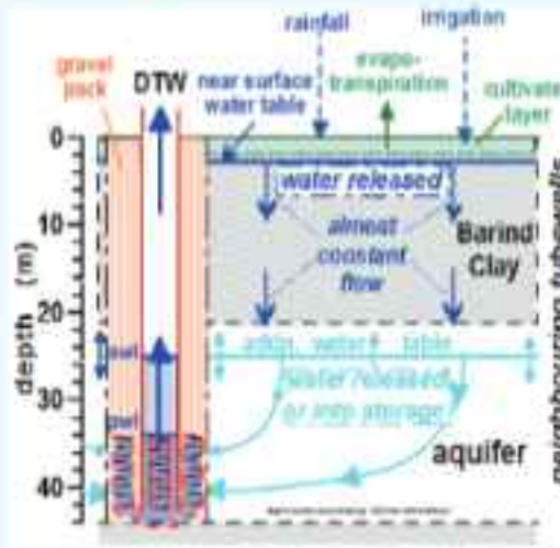
Fig. 2(b) current conditions rainfall and irrigation to cultivated layer evapotranspiration from cultivated layer water released from near surface water table almost constant flow through Barind Clay is less than pumping demand hence additional water table forms supplementary water released from additional water table beneath Clay elevation of static water level below Barind Clay; pumping water level within strainers
