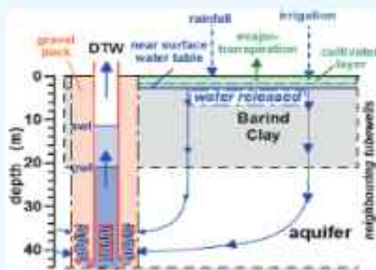
Fig. 2(a) early stages
