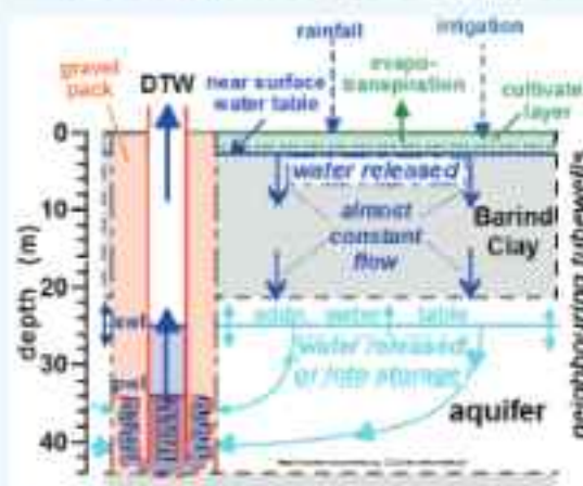
Fig. 2(b) current conditions
