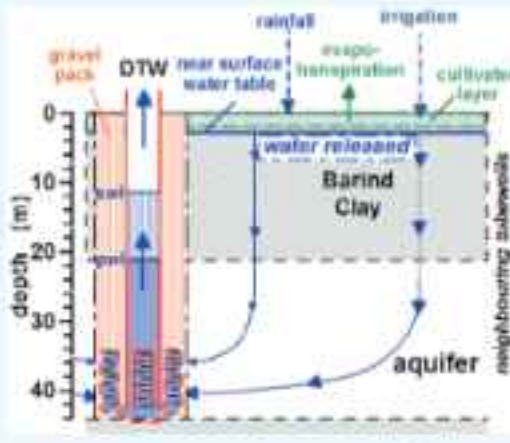
Fig. 2(a) early stages rainfall and irrigation to cultivated layer evapotranspiration from cultivated layer water released from near surface water table water drawn from near surface water table to well flows through the Barind Clay depth to static water level within Barind Clay; pumping water level above strainers
