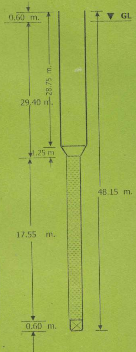
Cross Section of the Well (Not to scale)
