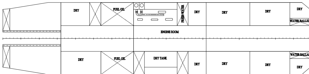
BOTTOM PLAN
