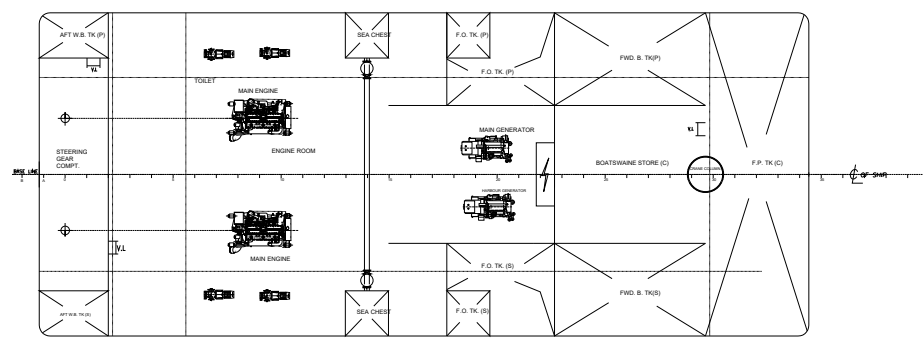
BELOW MAIN DECK PLAN
