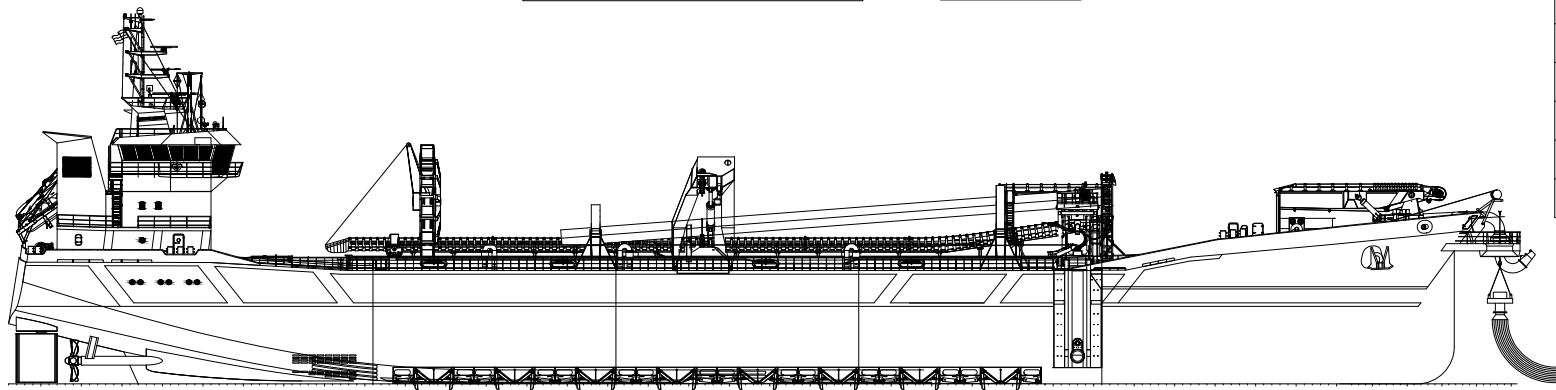
PROFILE
