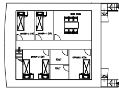
POOP DECK
