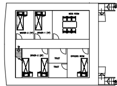
POOP DECK
