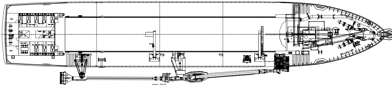
MAIN DECK
