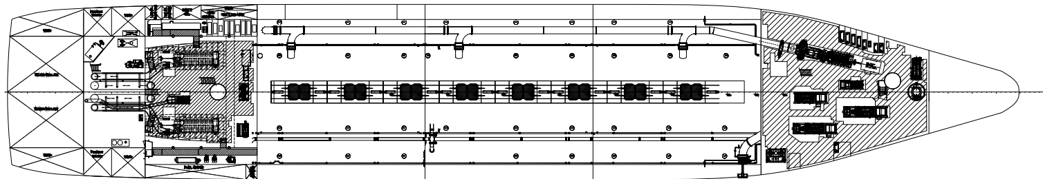
UNDER DECK
