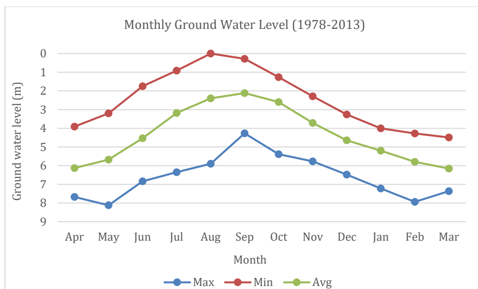
Figure 5.33: Depth of Groundwater at Sirajganj Station
