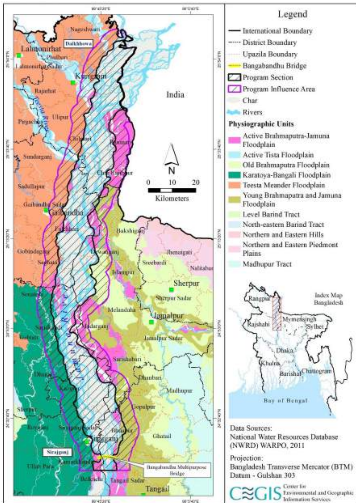
Figure 5.5: The Physiographic Units of the Program AOI and EBAA
