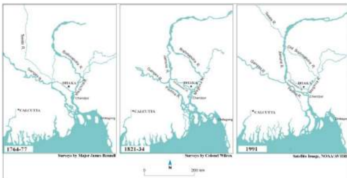
Figure 5.11: Historical Development of the Brahmaputra-Jamuna River
