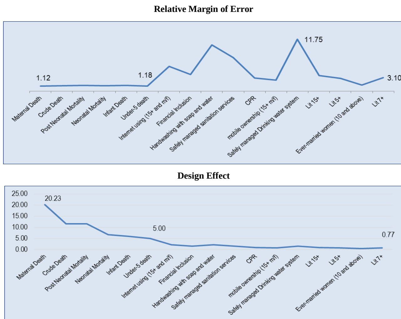
Figure 3.2: RME and Design Effect for Different Indicators: PSU size 25
