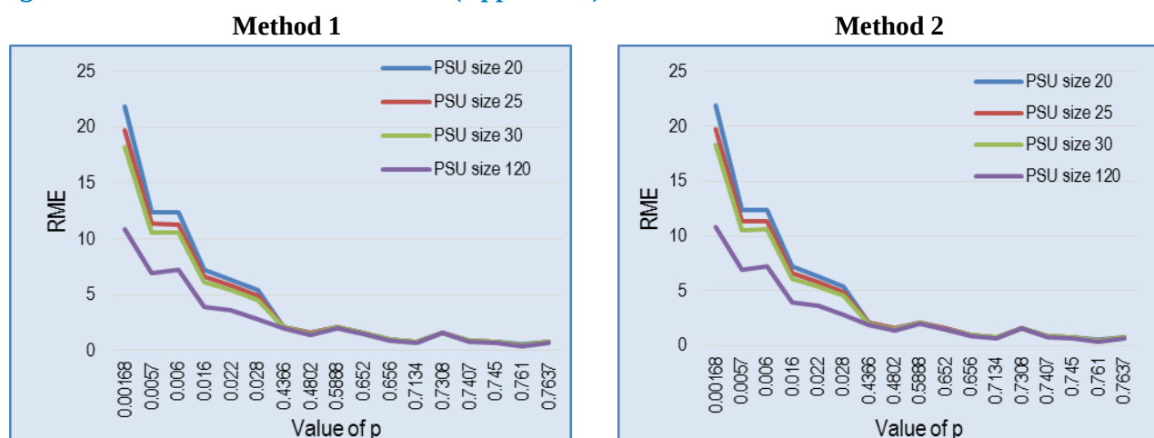
Figure 3.3: RME for Different PSU size (Approach I)
