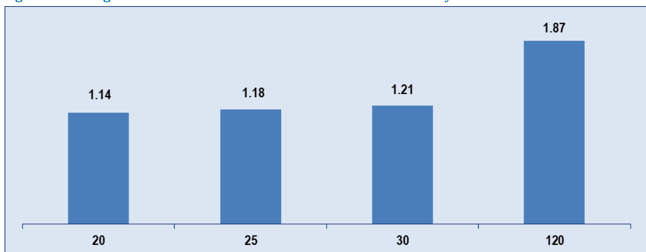
Figure 3.1: Design Effect for Different PSU Size for Under-5 Mortality Rate
