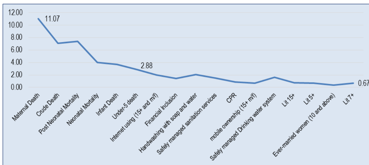
Figure 3.8: RME variation for different indicators, different levels of delineation by Approach II
