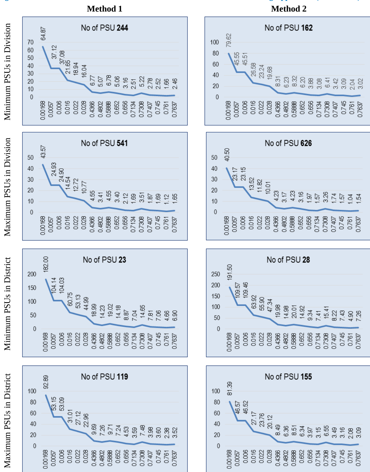
Figure 3.4: RME for minimum and maximum PSUs in division and districts using Approach I (PSU size 25)
