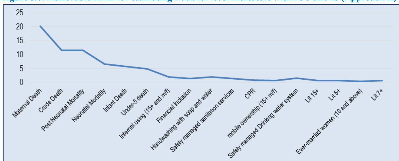
Figure 3.7: RME for Different Indicators at Division and District Level by Approach II: PSU size 25
