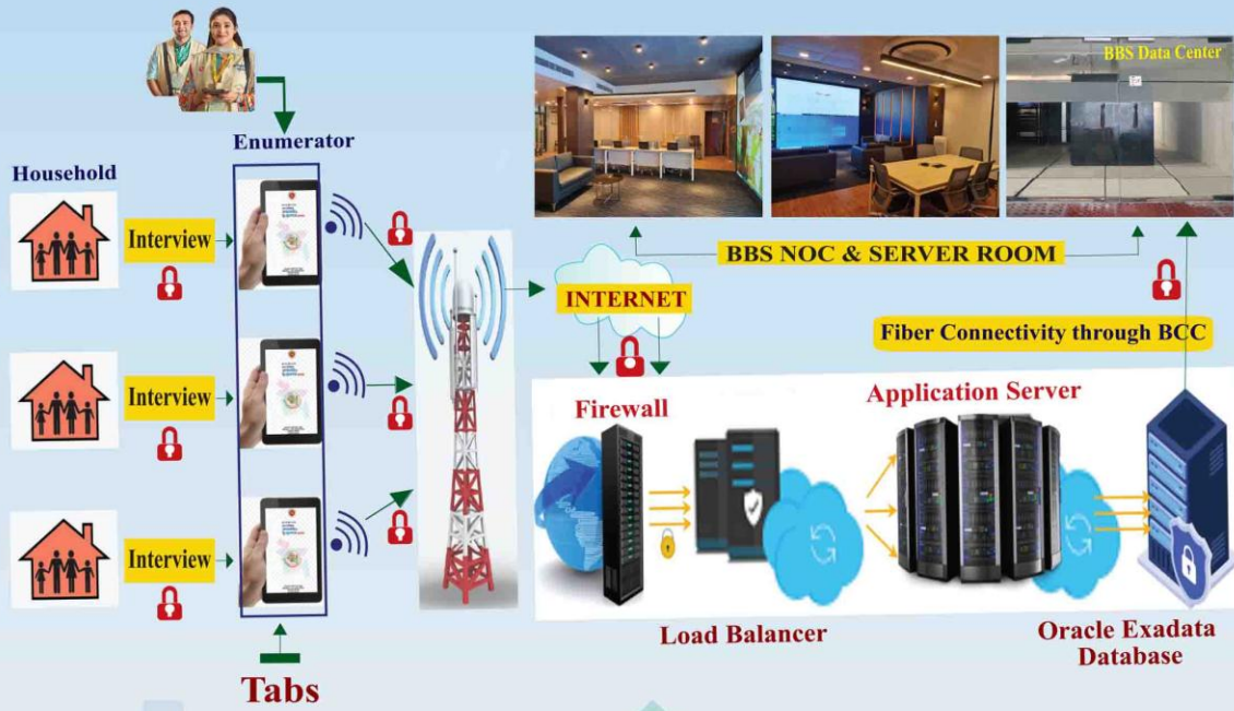
The ICT Architecture of Population and Housing Census 2022
