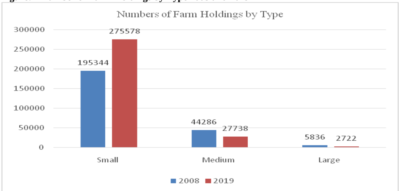
Figure: 2 Number of Farm Holdings by Type 2008 and 2019
