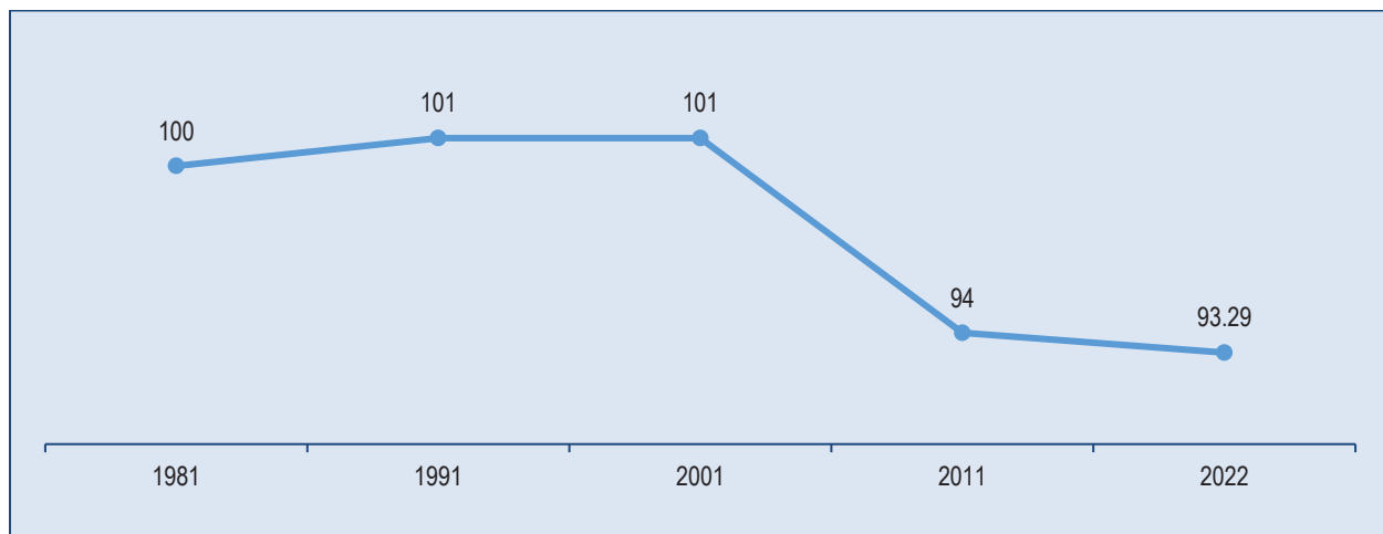
Figure 3.1.5 Sex Ratio, 1981-2022
