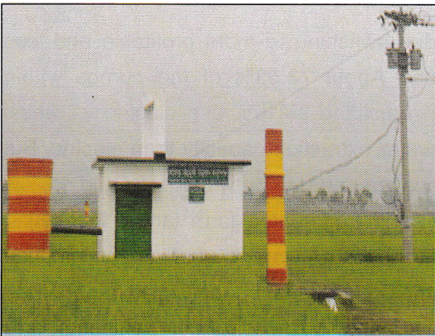
Figure 7: BMDA DTW in Taraganj, Rangpur Upazila
