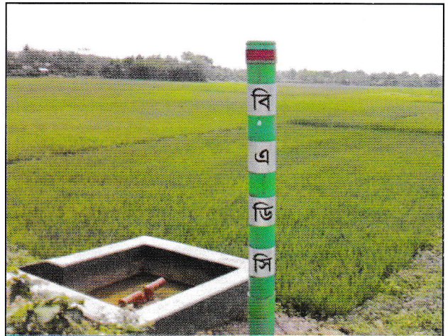
Figure 6: Electrically Operated Deep Tube Well and Buried Pipe Line.
